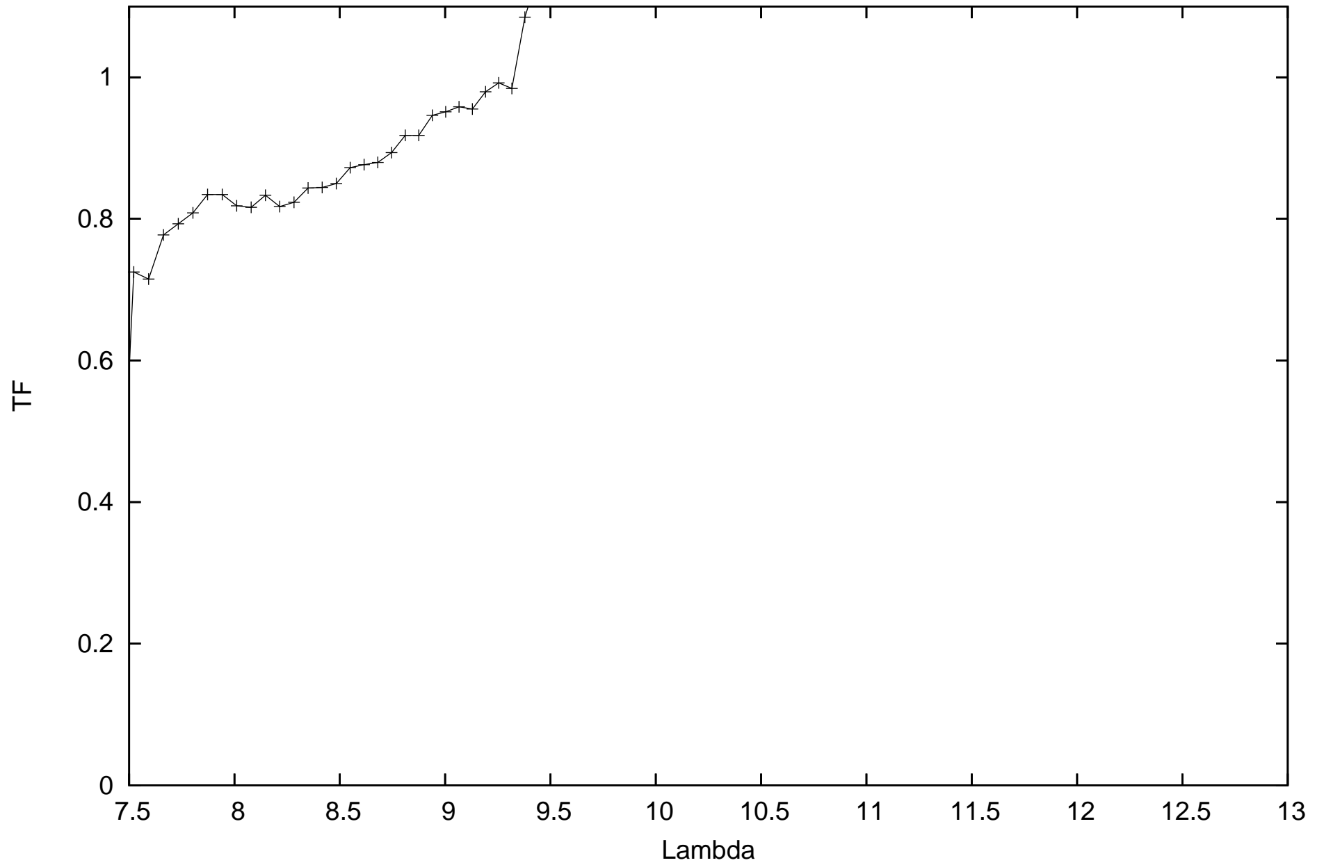
calHIP9347_flux-0.13268_diam5.836626_r.MIDI.2013-09-11T08_26_02.000_D0B2
