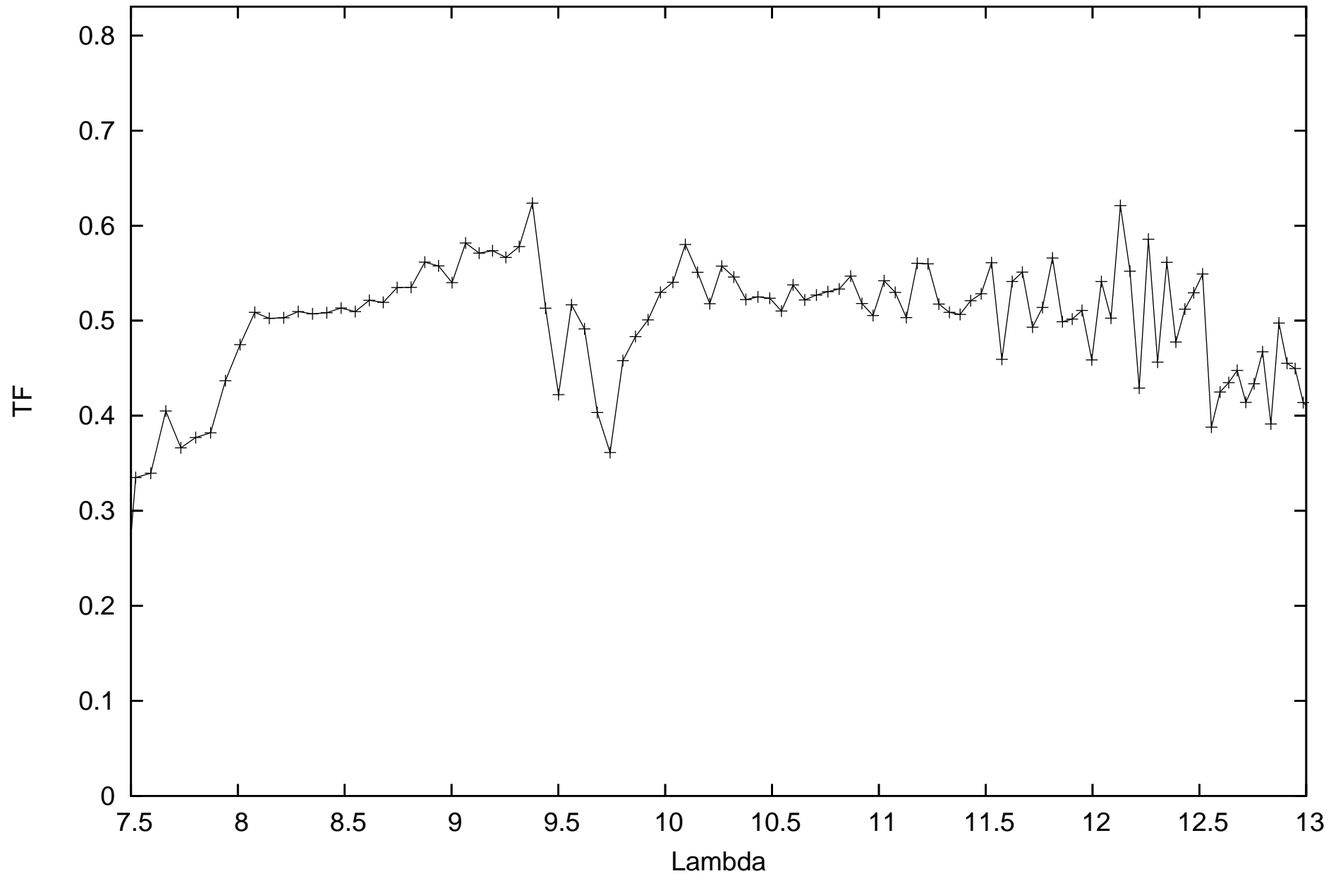
calHIP90496_flux0.238088_diam3.99_r.MIDI.2013-09-17T04_04_14.000_H011
