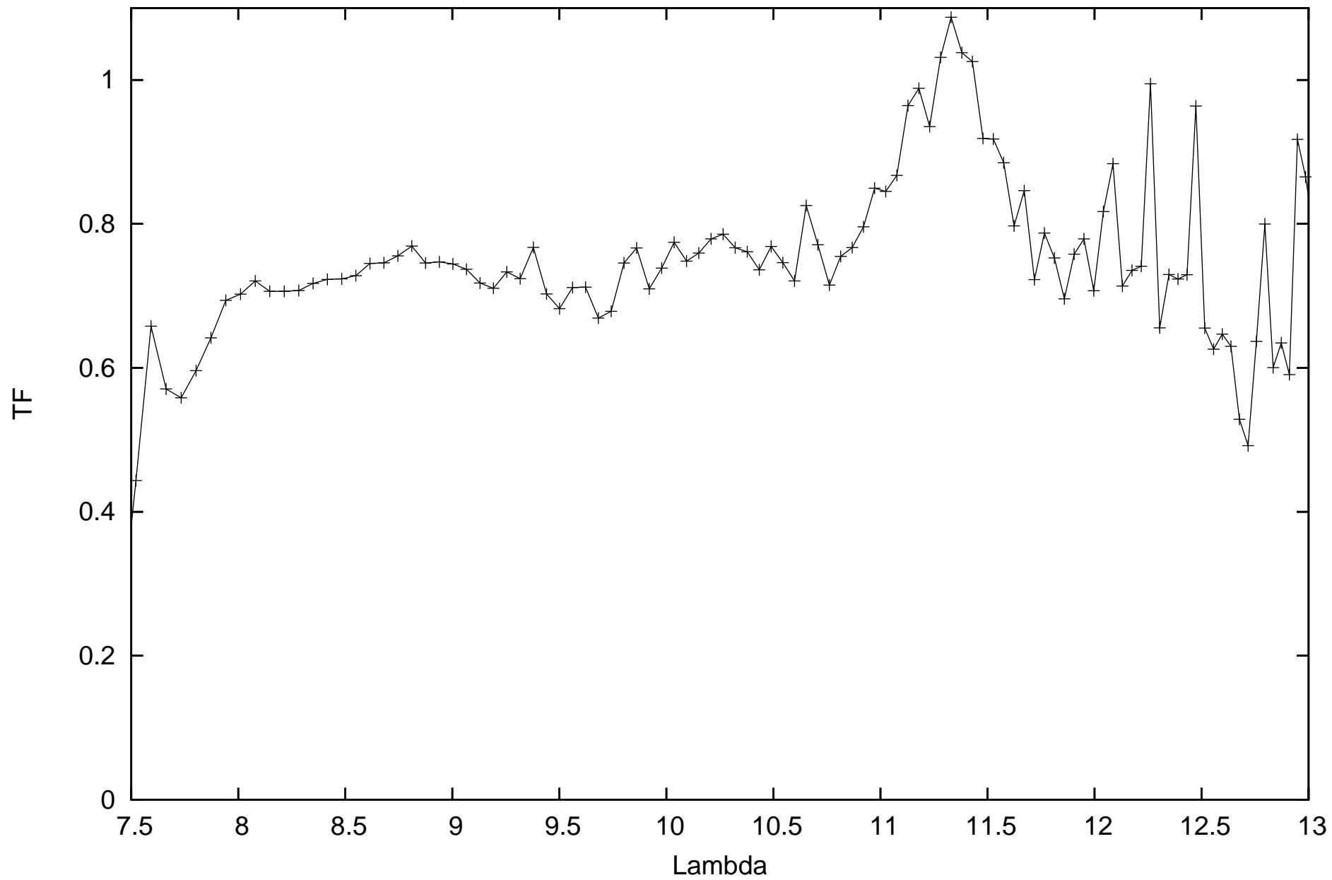
calHIP90496_flux0.238088_diam3.99_r.MIDI.2013-09-06T00_09_42.000_K0G1
