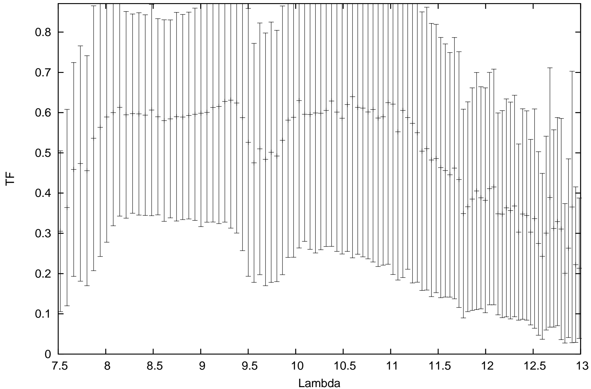
calHIP90496_flux0.238088_diam3.99_r.MIDI.2013-09-05T23_31_27.000_K0G1
