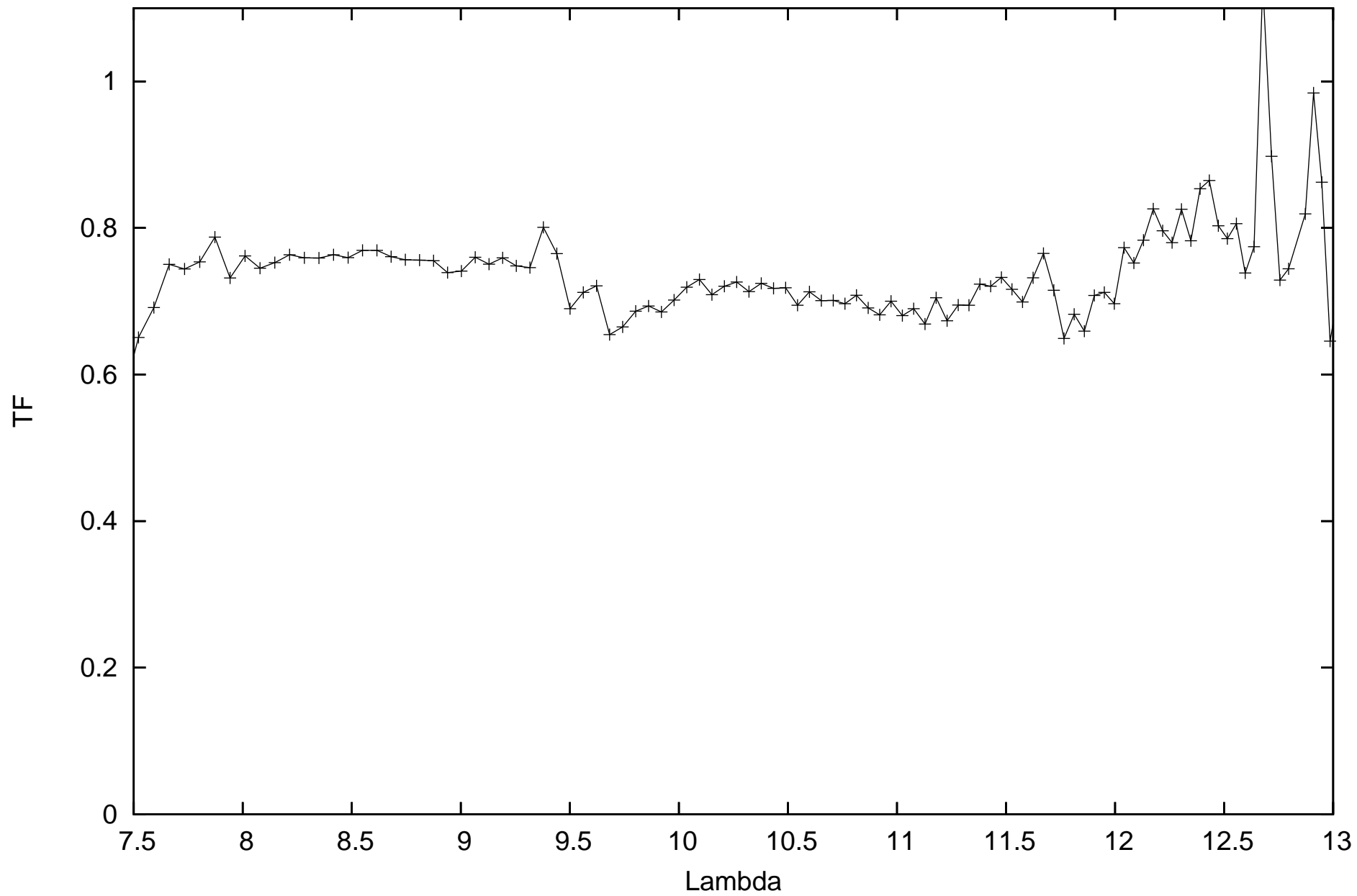
calHIP90496_flux0.238088_diam3.99_r.MIDI.2013-08-15T06_06_46.000_G111
