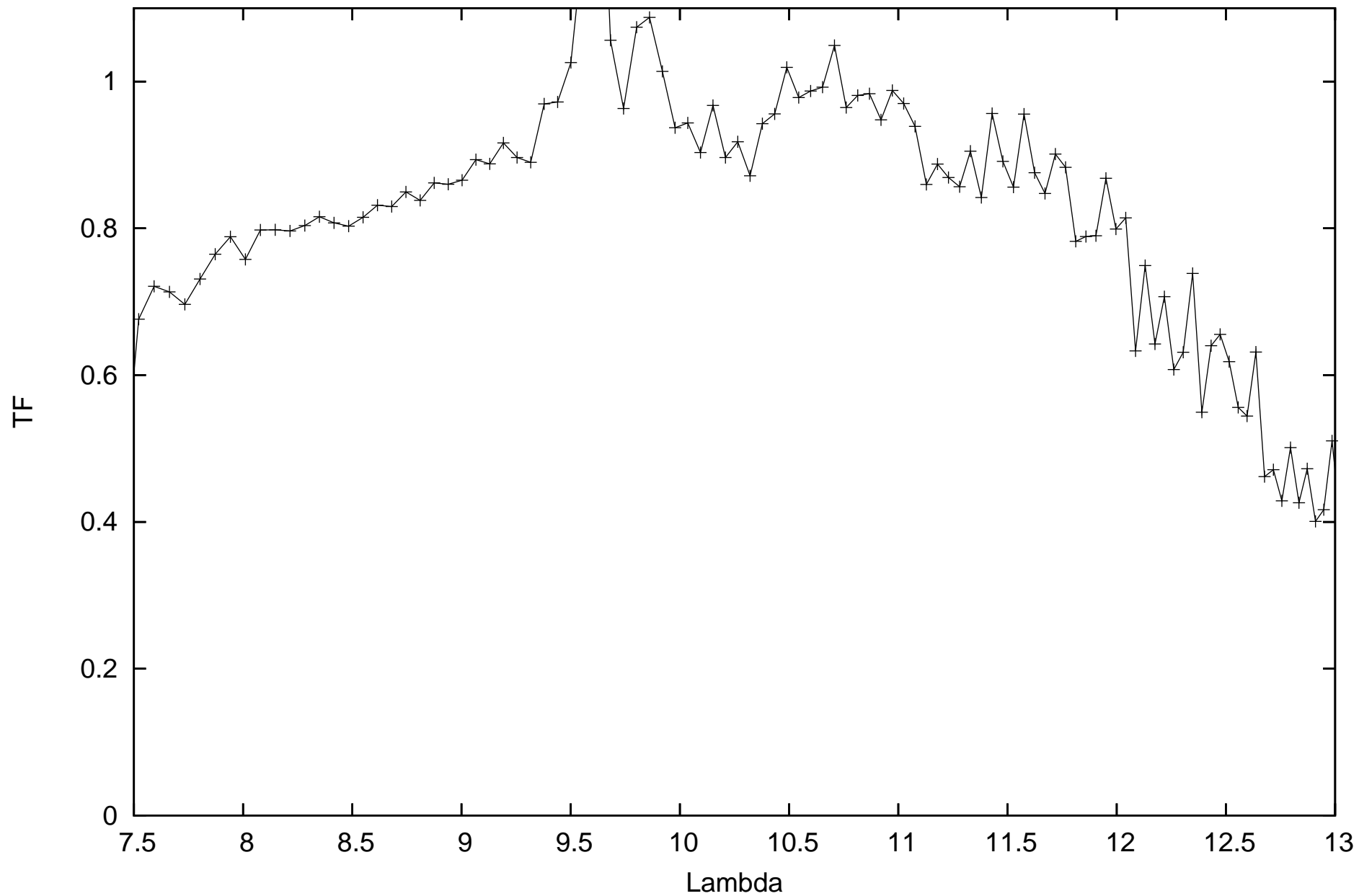
calHIP90496_flux0.238088_diam3.99_r.MIDI.2013-07-16T07_23_03.000_D0G1
