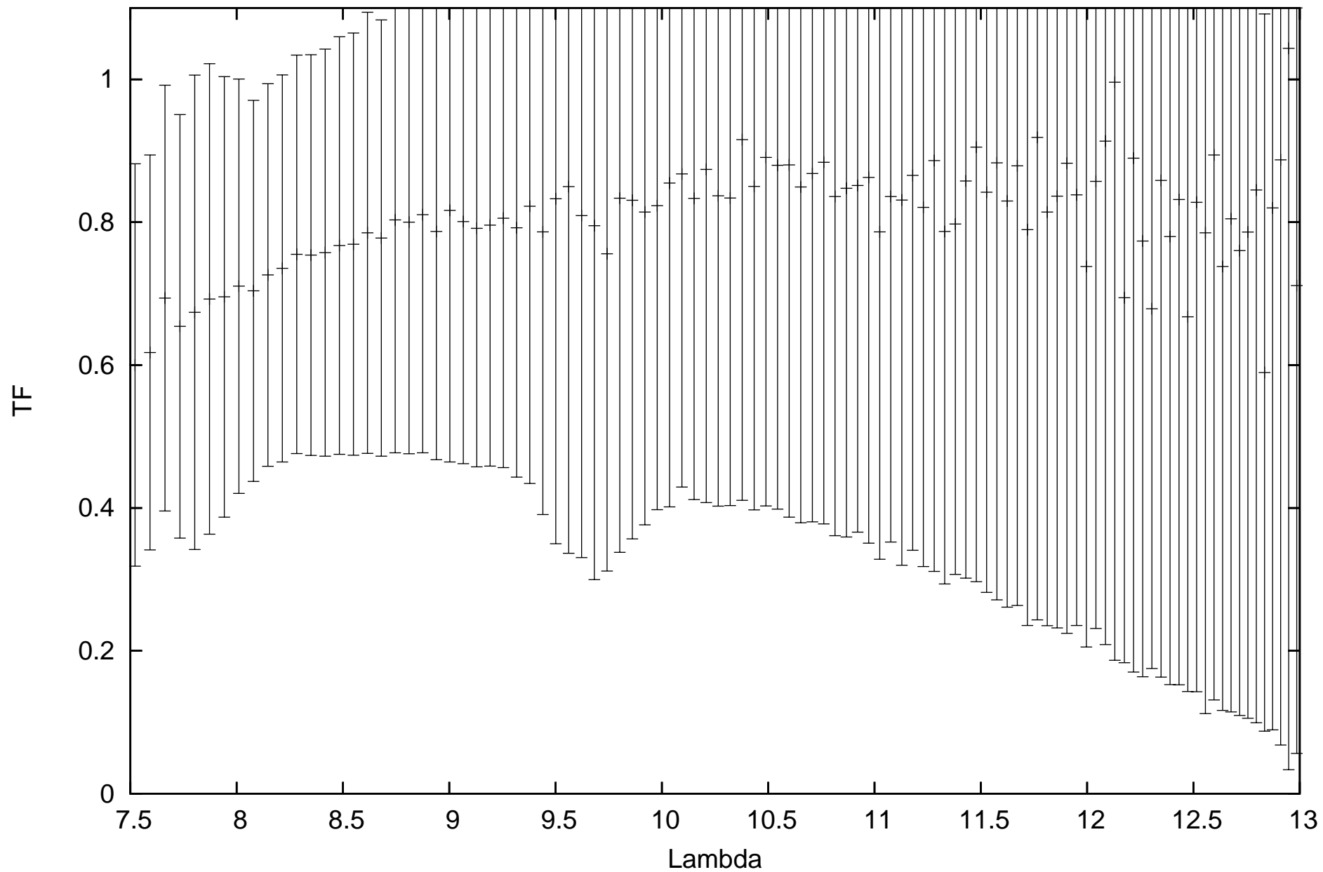
calHIP90496_flux0.238088_diam3.99_r.MIDI.2013-07-16T05_51_00.000_H0G1
