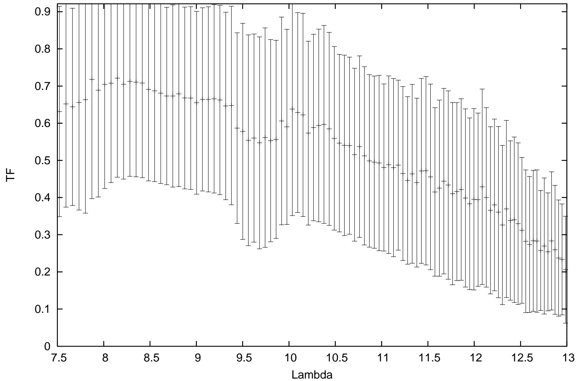
calHIP90496_flux0.238088_diam3.99_r.MIDI.2013-07-16T02_37_11.000_D0H0
