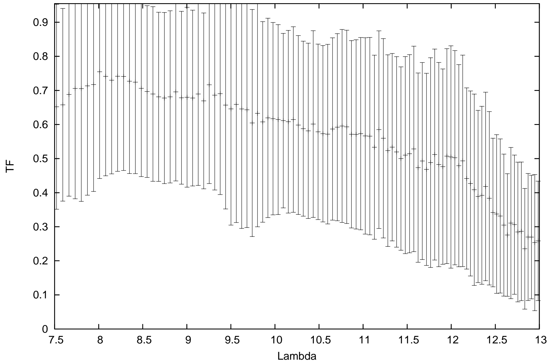
calHIP90496_flux0.238088_diam3.99_r.MIDI.2013-07-16T02_07_13.000_D0H0
