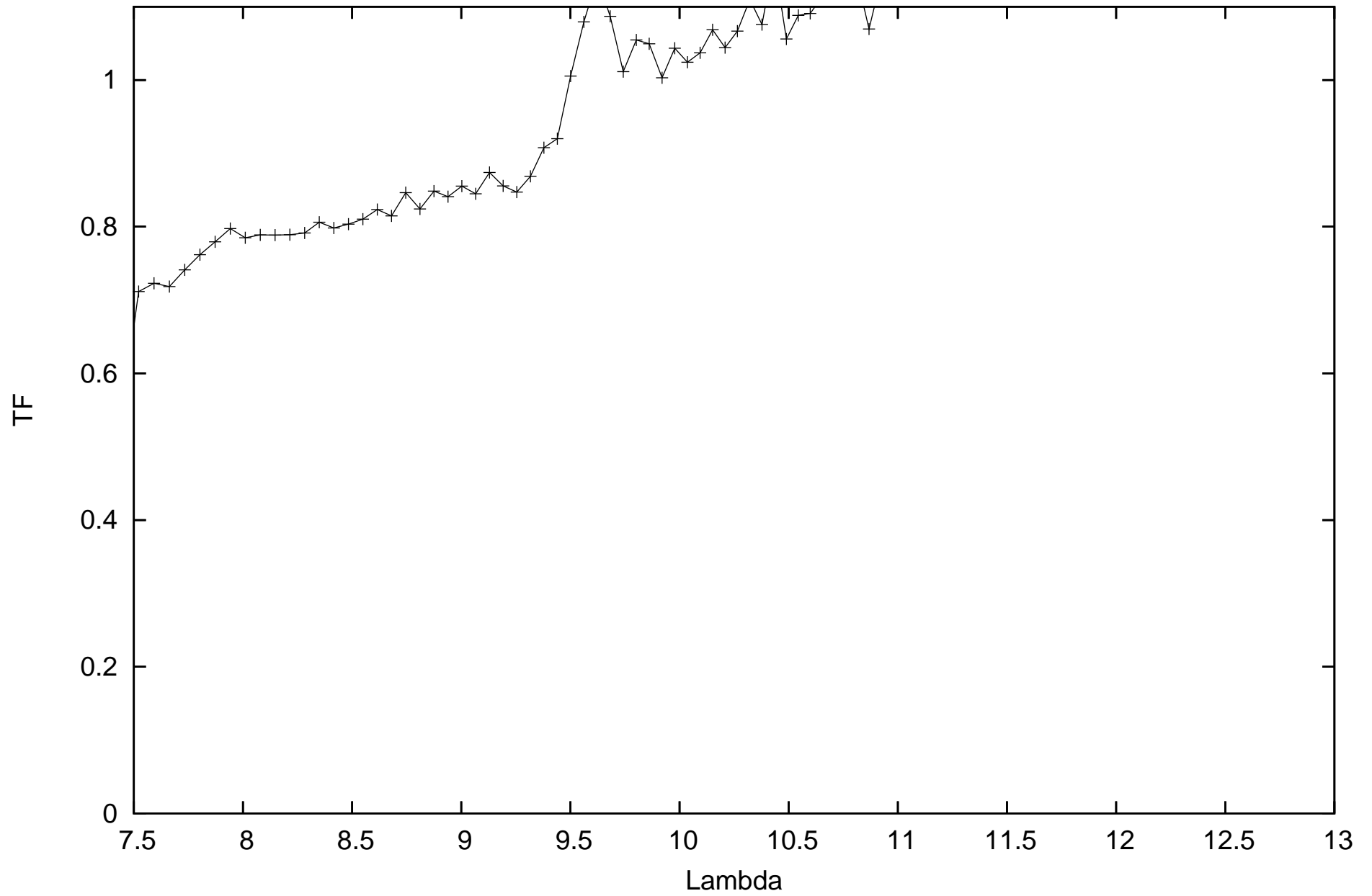
calHIP90496_flux0.238088_diam3.99_r.MIDI.2013-07-12T05_36_35.000_K0J3
