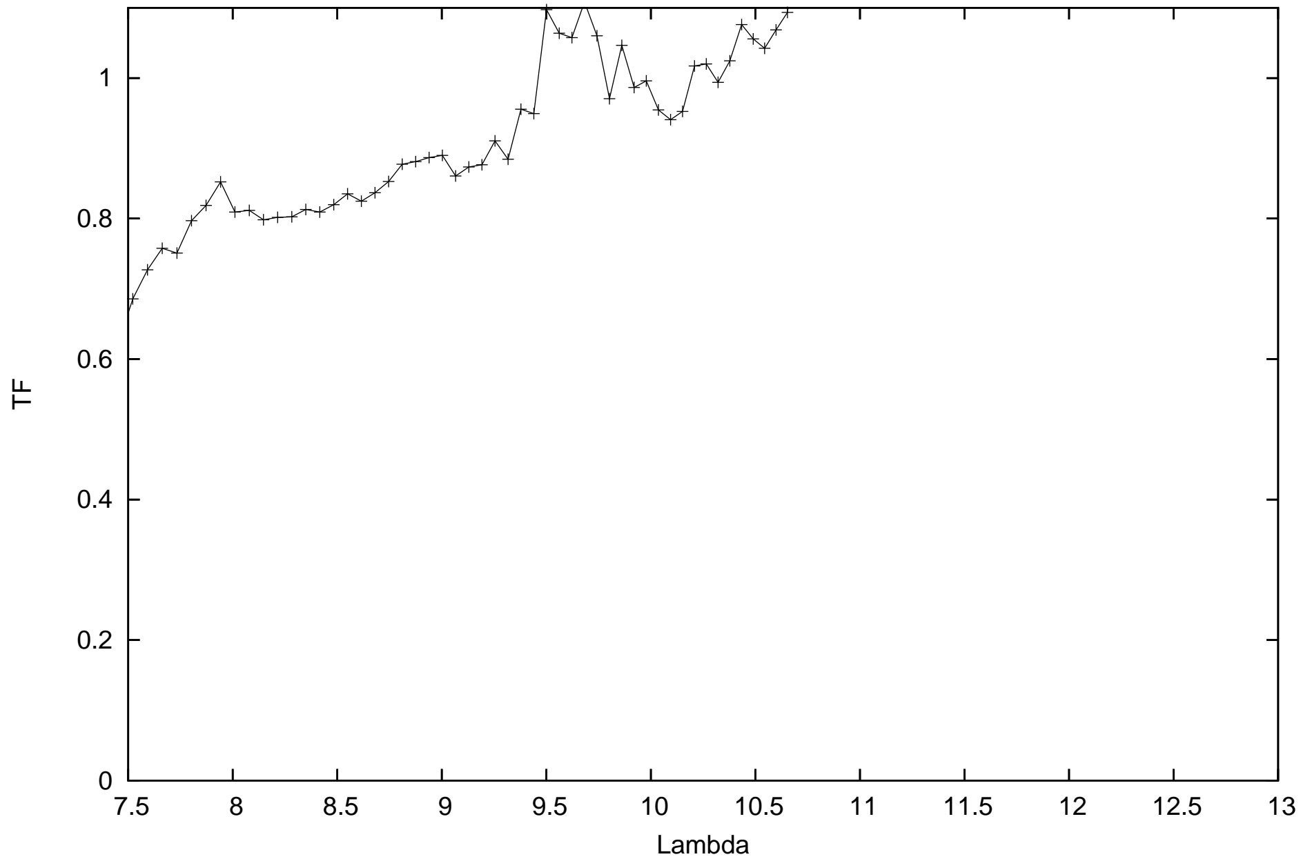
calHIP90496_flux0.238088_diam3.99_r.MIDI.2013-07-12T05_12_23.000_K0J3
