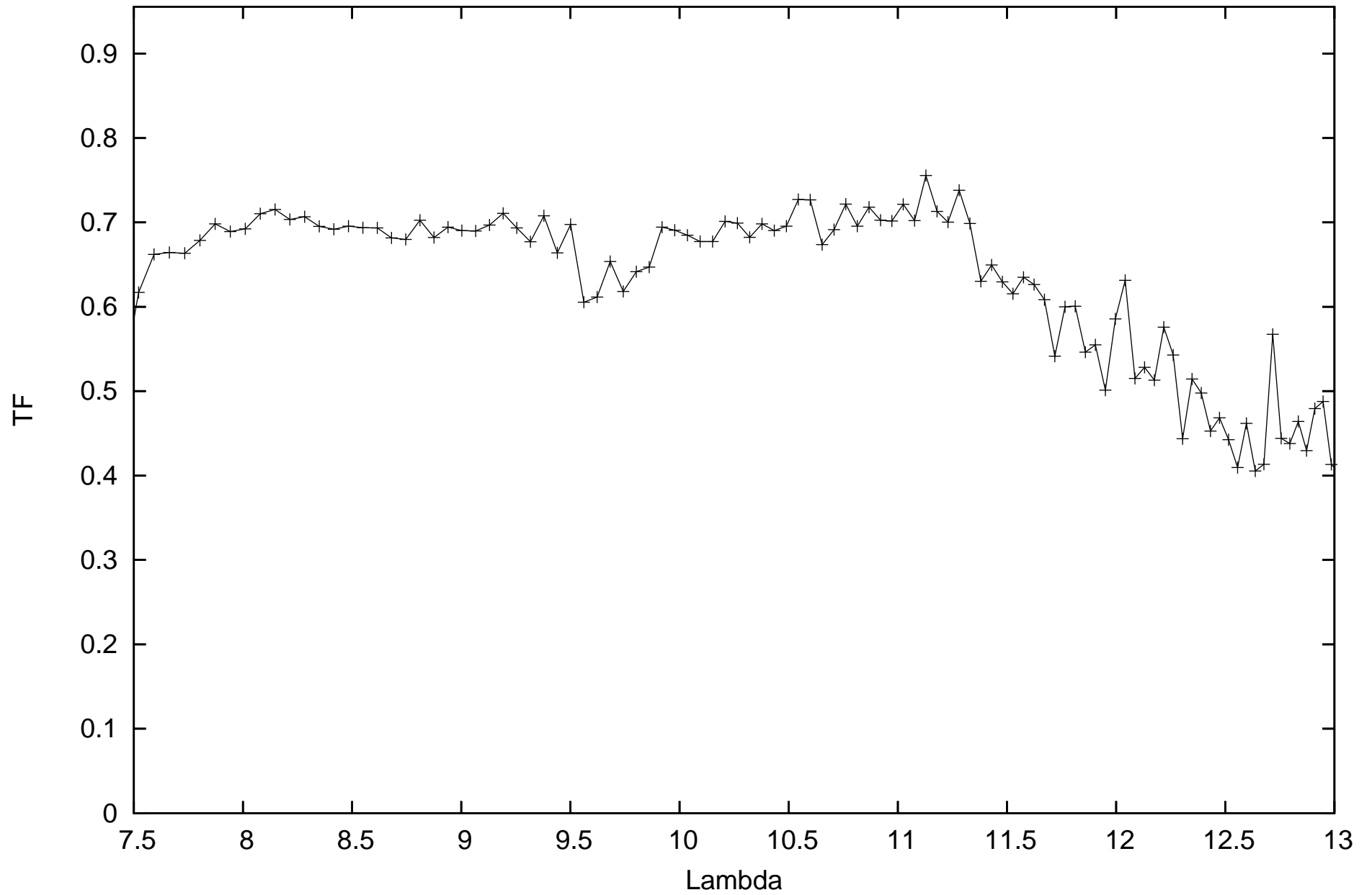
calHIP90496_flux0.238088_diam3.99_r.MIDI.2013-07-12T03_08_50.000_G1A1
