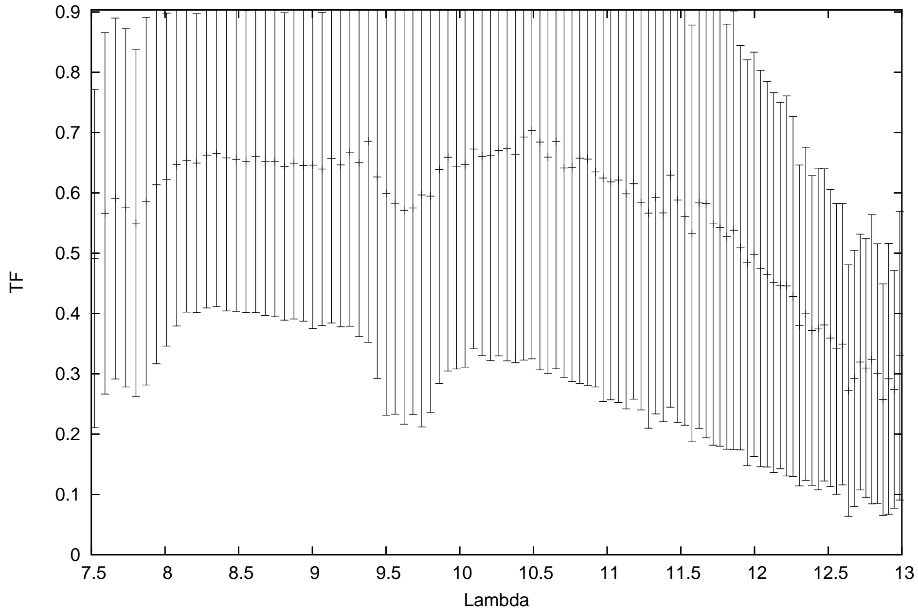
calHIP90496_flux0.238088_diam3.99_r.MIDI.2013-07-12T01_52_49.000_K0G1
