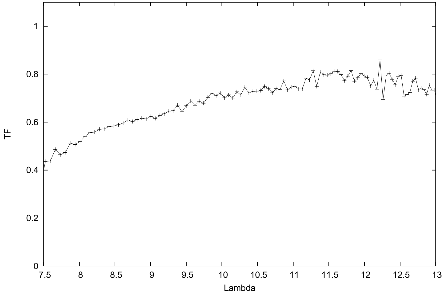
calHIP89931_flux-0.511_diam5.87_r.MIDI.2013-05-12T09_39_35.000_C1A1
