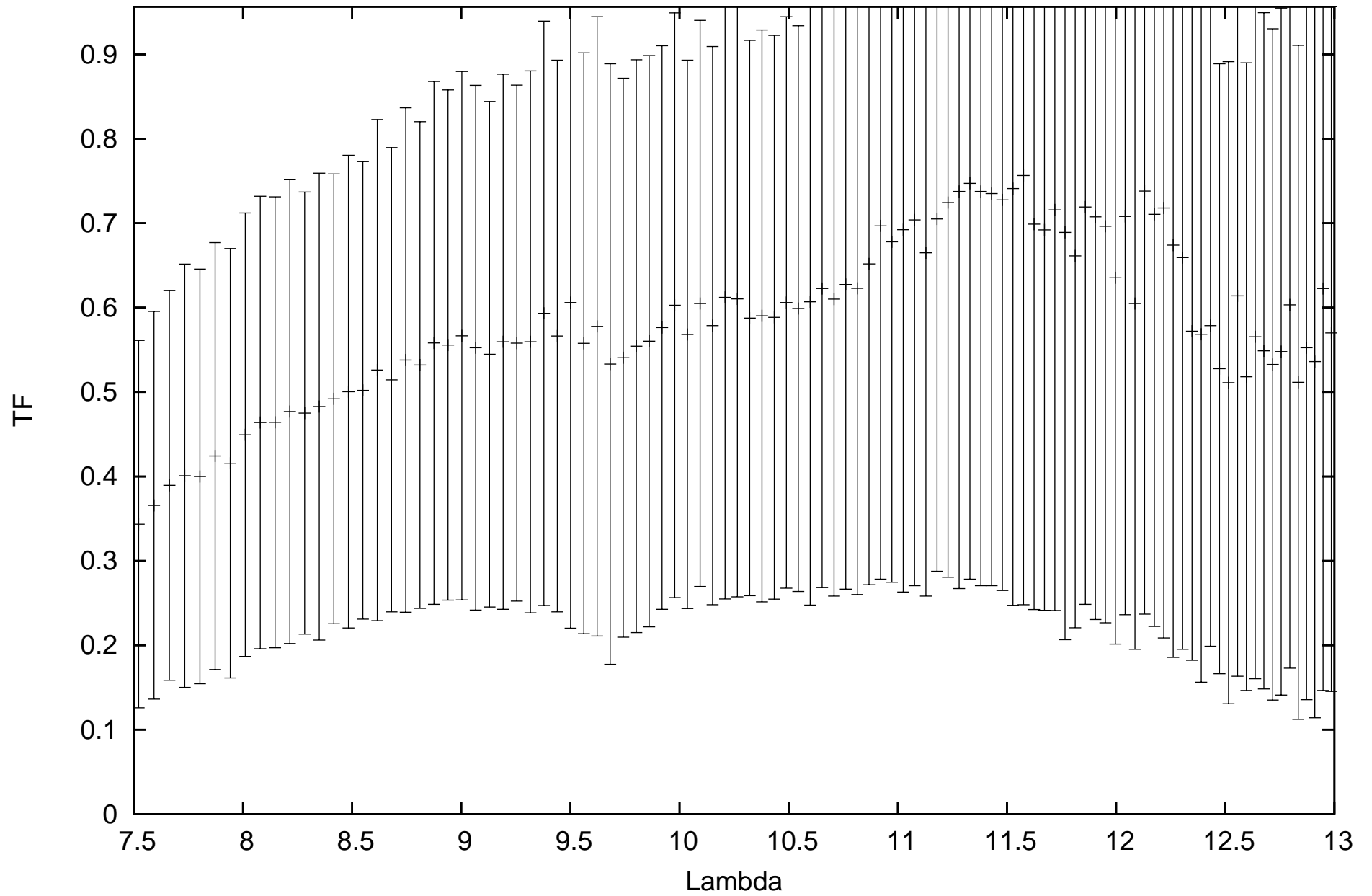
calHIP89931_flux-0.511_diam5.87_r.MIDI.2013-05-12T09_12_42.000_D0B2
