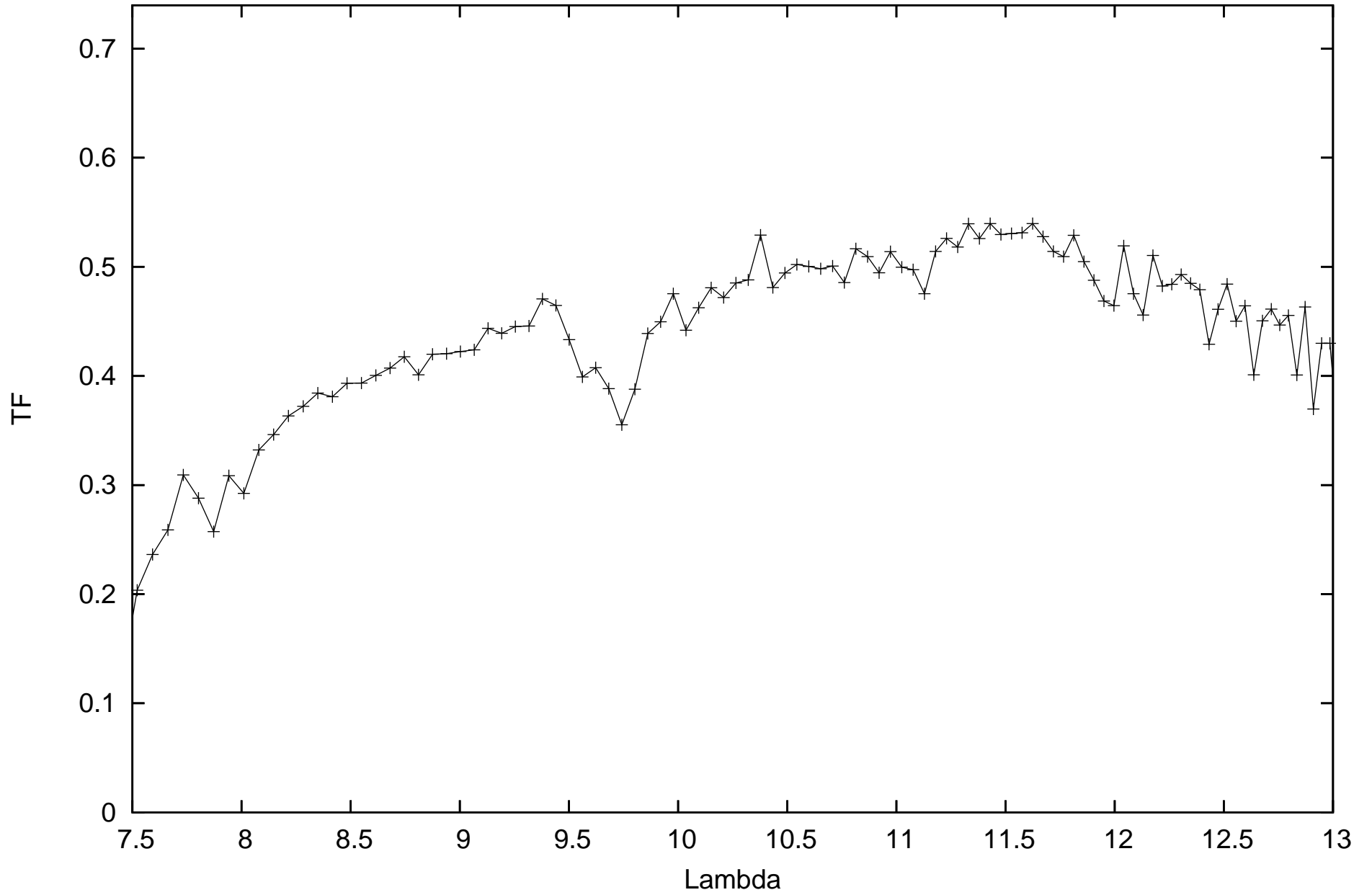
calHIP89683_flux1.83165_diam2.196101_r.MIDI.2013-06-21T03_55_42.000_U1U4
