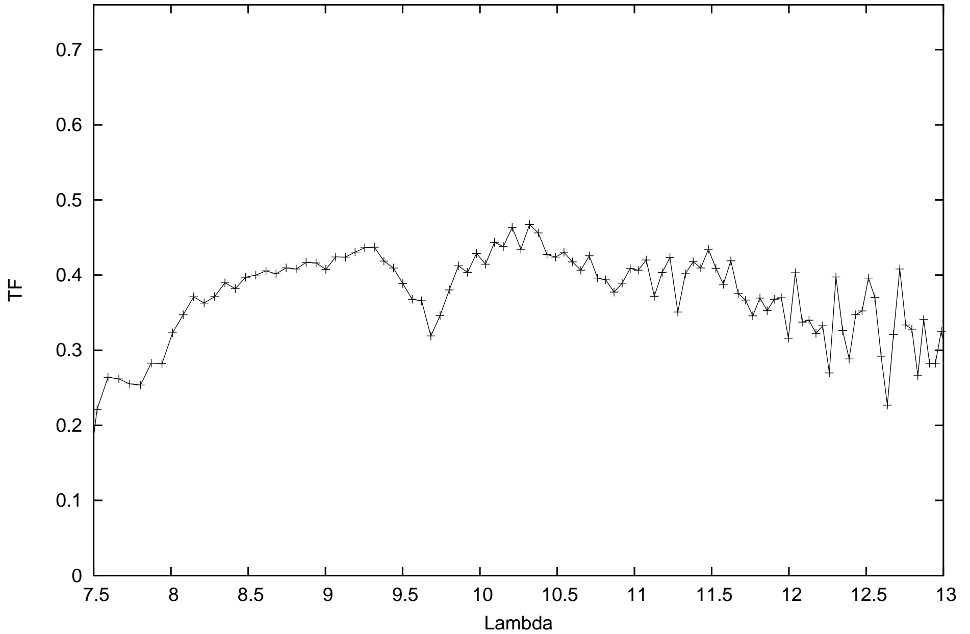
calHIP87540_flux3.35354_diam0.901651_r.MIDI.2013-05-28T05_25_33.000_U1U4
