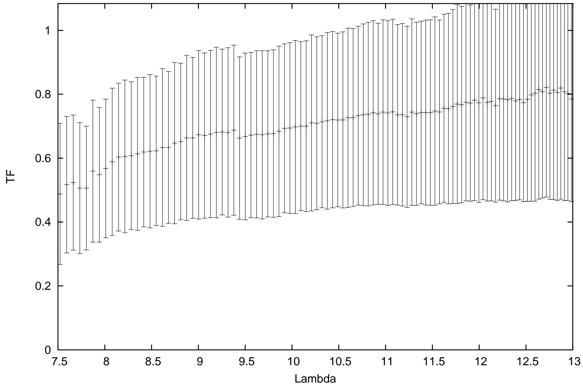
calHIP7588_flux0.936365_diam1.68_r.MIDI.2013-12-17T01_17_28.000_U2U4
