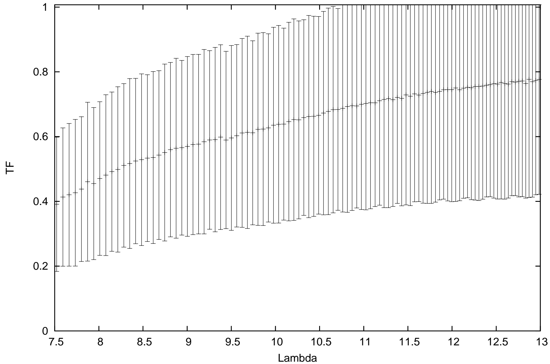
calHIP73714_flux-1.78451_diam11.15_r.MIDI.2013-06-19T01_05_08.000_U2U3
