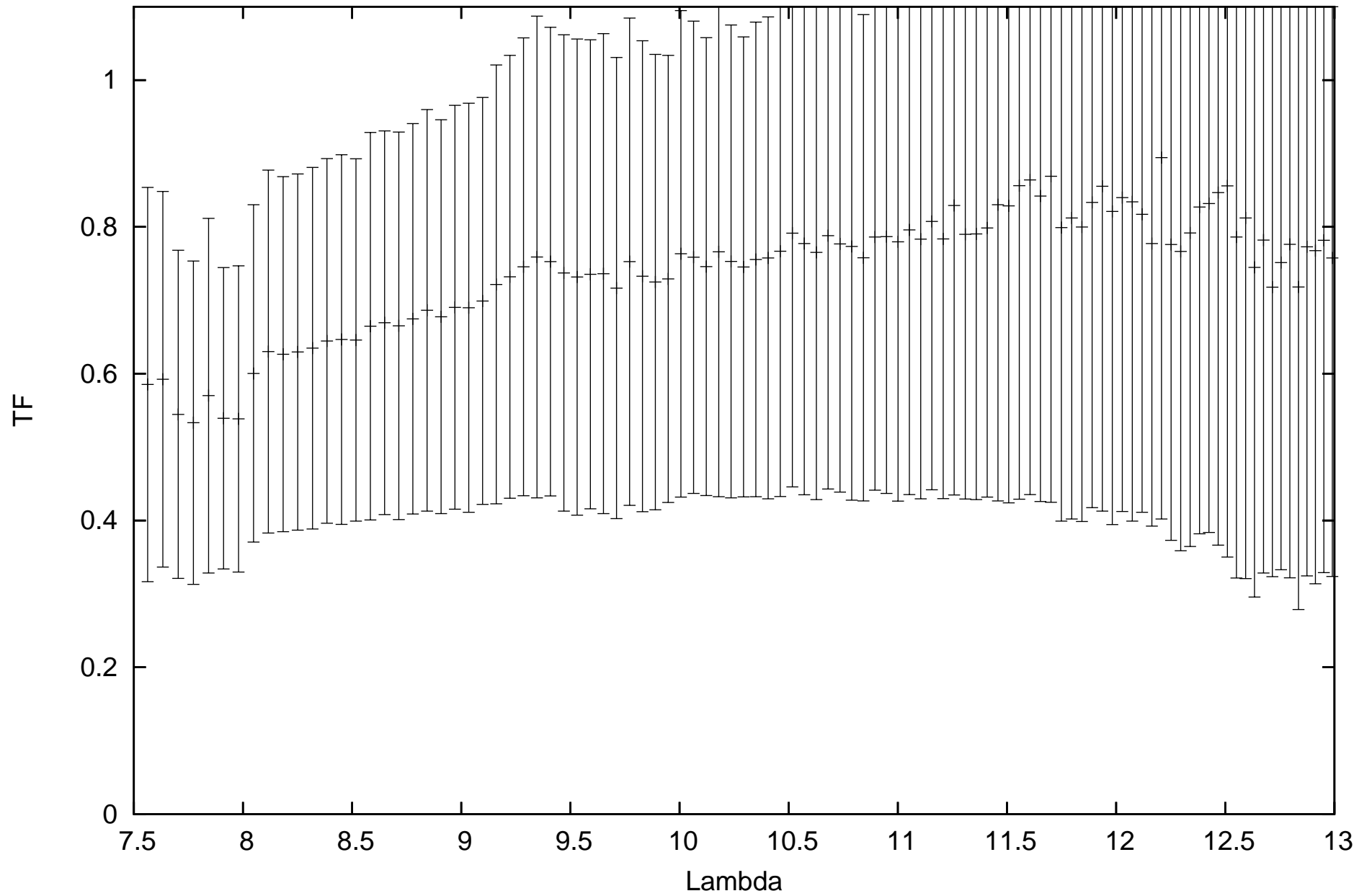
calHIP73714_flux-1.78451_diam11.15_r.MIDI.2013-04-07T05_16_09.112_D0H0
