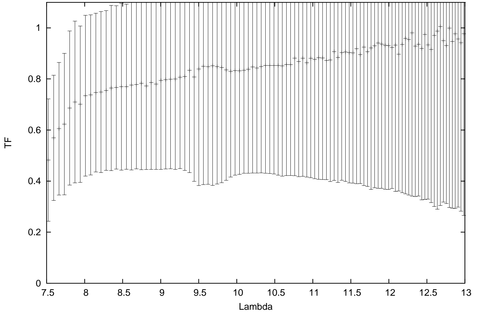
calHIP64117_flux1.55227_diam2.637496_r.MIDI.2013-03-02T09_25_40.000_U1U3
