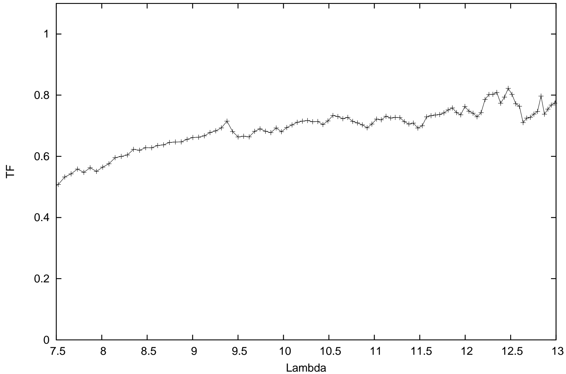
calHIP57047_flux1.57349_diam2.35_r.MIDI.2013-06-23T00_55_02.000_U2U3
