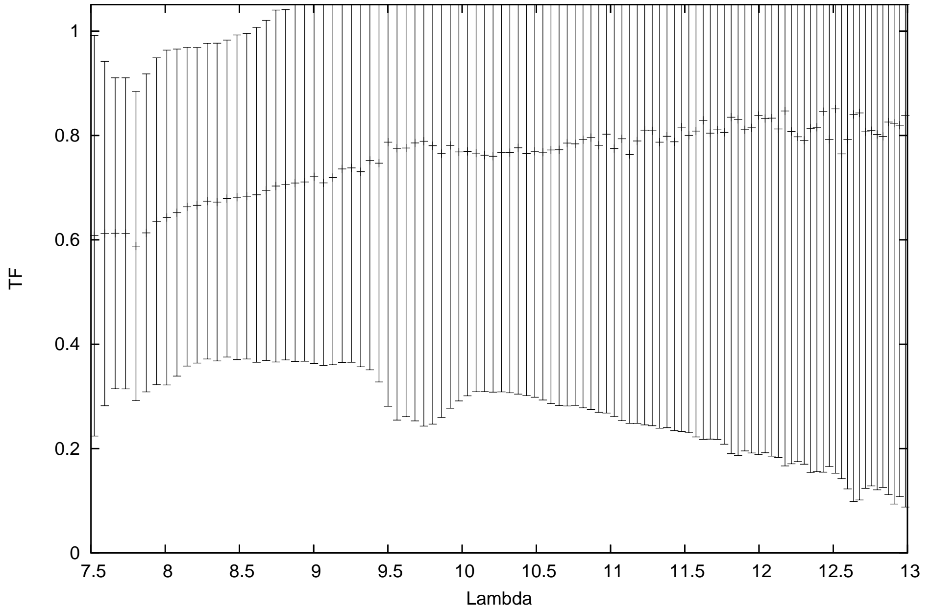
calHIP27938_flux1.62718_diam2.214782_r.MIDI.2013-12-15T06_00_35.000_U1U2
