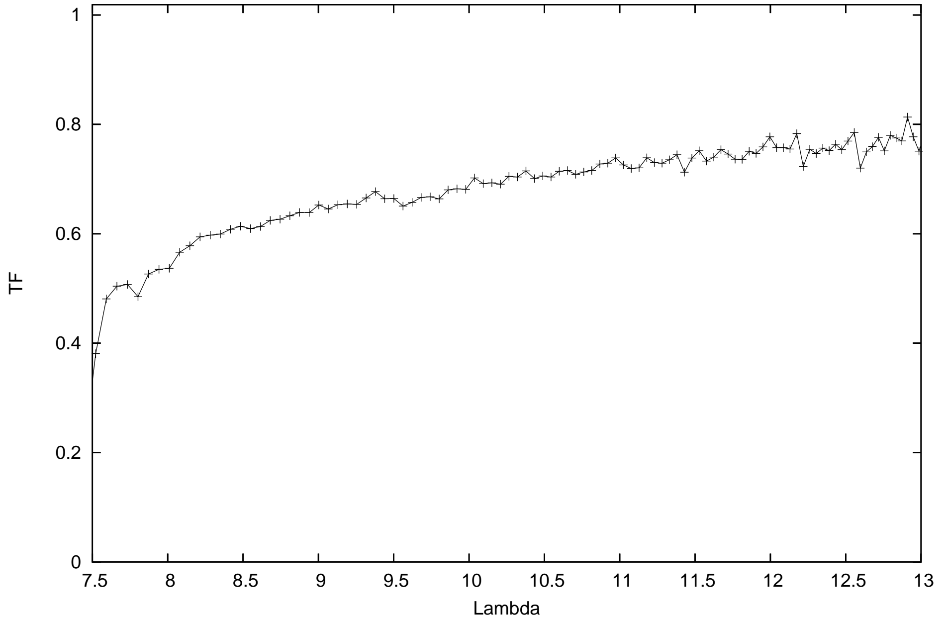
calHIP27938_flux1.62718_diam2.214782_r.MIDI.2013-12-15T05_19_19.000_U1U2
