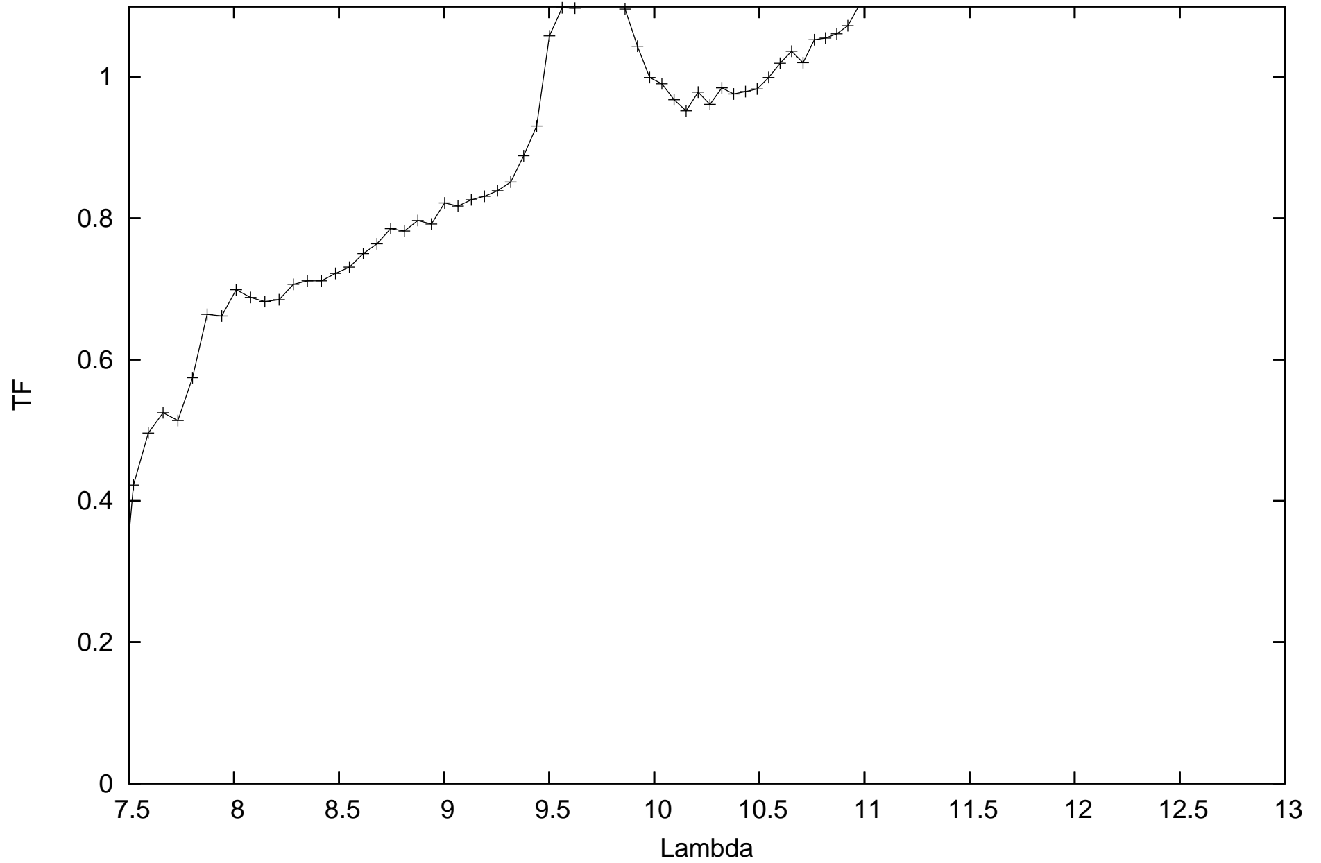
calHIP27938_flux1.62718_diam2.214782_r.MIDI.2013-12-14T05_19_15.000_U3U4
