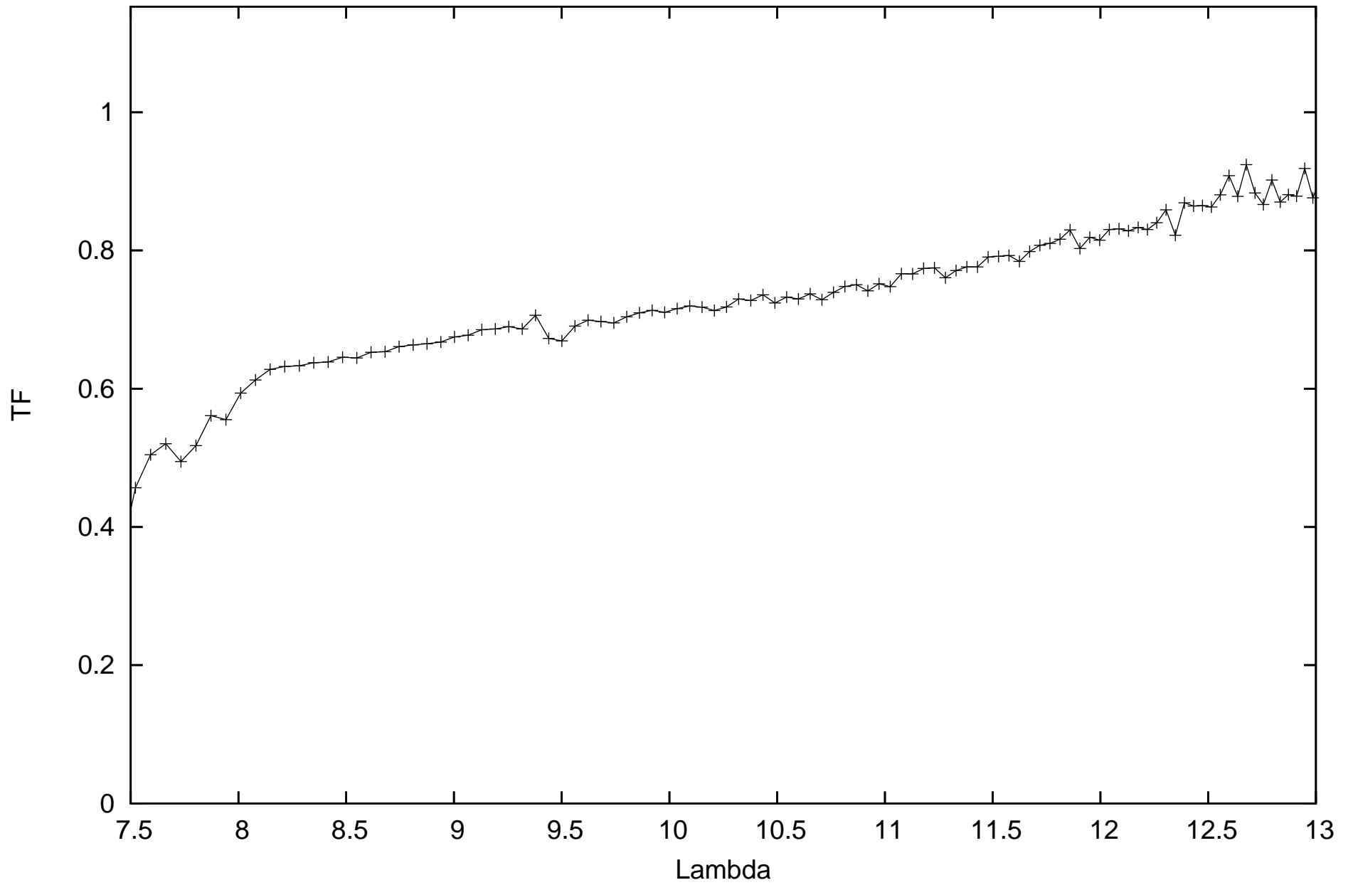
calHIP27938_flux1.62718_diam2.214782_r.MIDI.2013-12-14T04_29_07.000_U3U4
