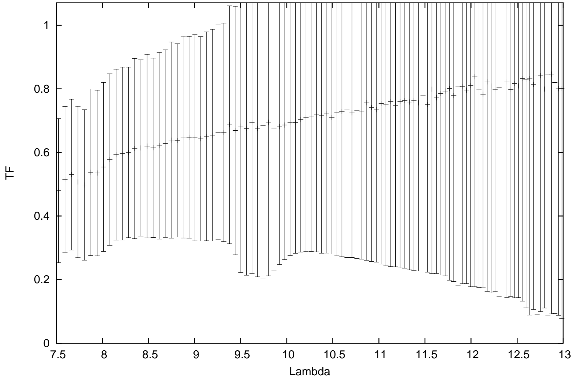
calHIP27938_flux1.62718_diam2.214782_r.MIDI.2013-12-14T01_49_32.000_U3U4
