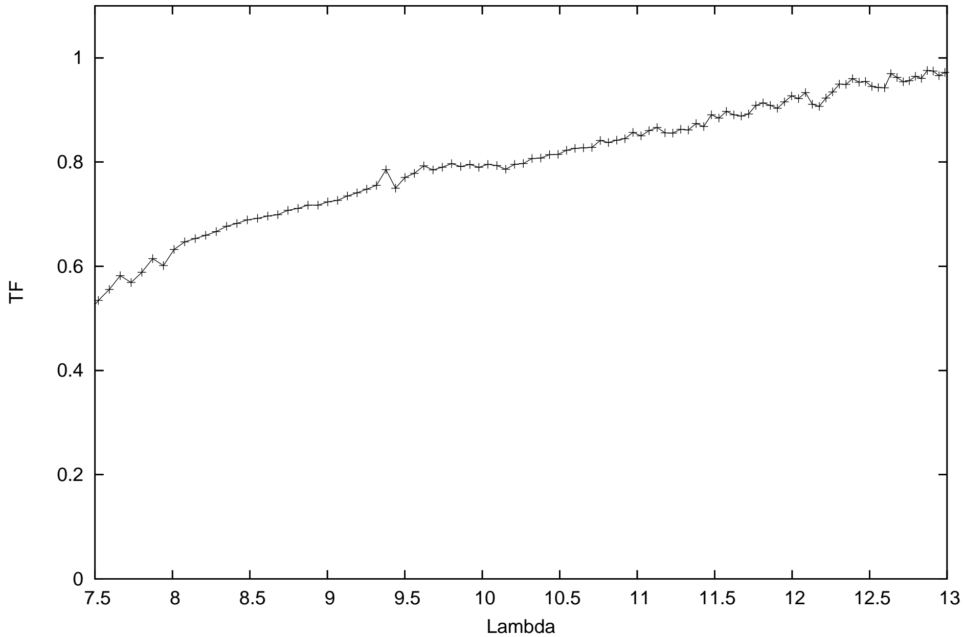
calHIP25859_flux1.10043_diam2.66_r.MIDI.2013-10-20T05_04_52.000_U1U3
