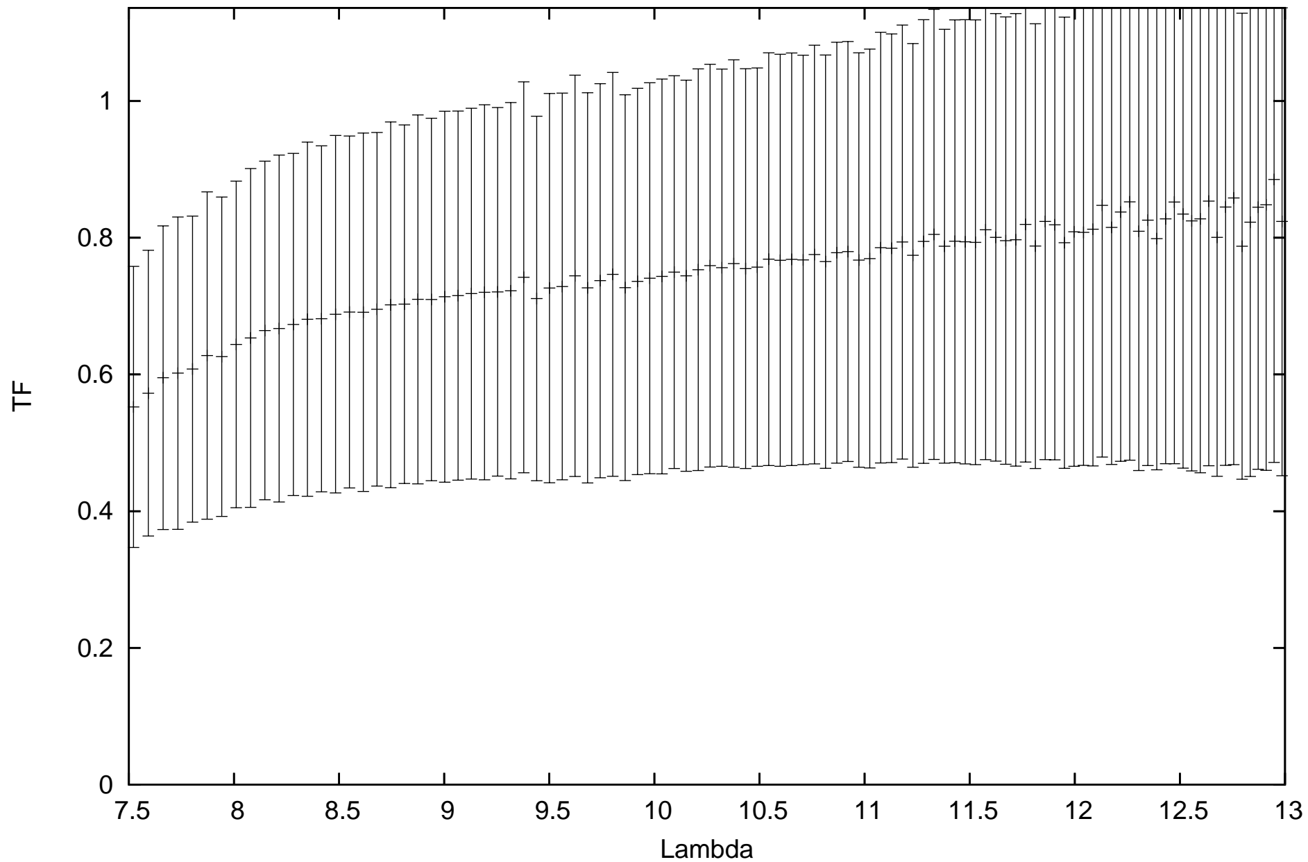
calHIP25859_flux1.10043_diam2.66_r.MIDI.2013-10-19T05_48_11.000_U1U4
