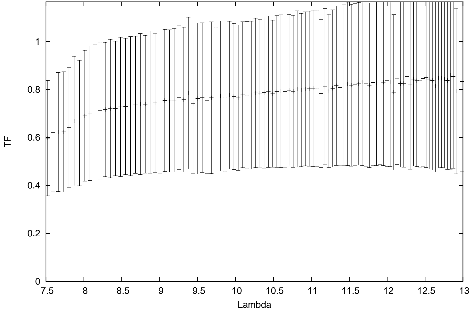
calHIP24197_flux1.37991_diam2.442016_r.MIDI.2013-10-21T05_34_22.000_U3U4
