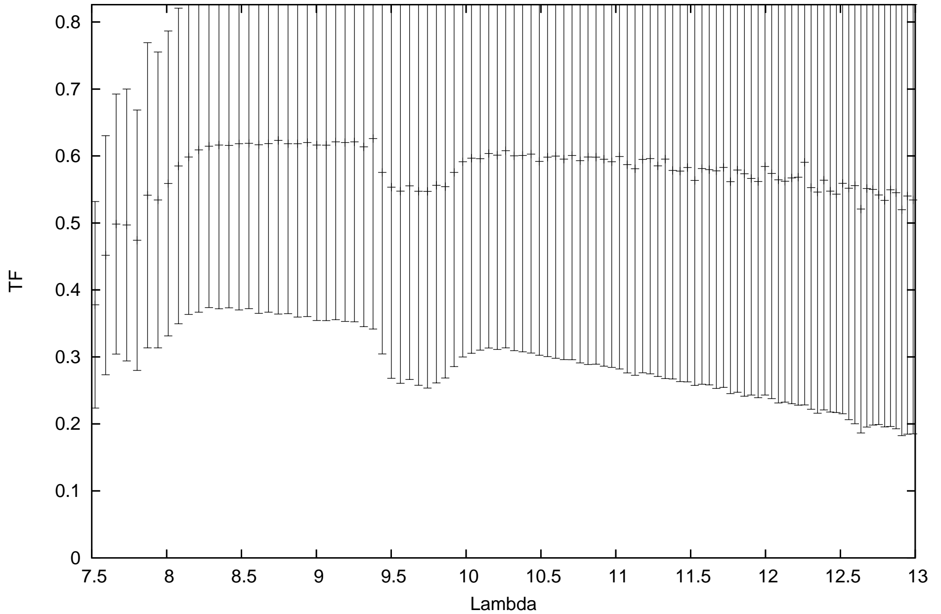
calHIP19038_flux1.83316_diam1.9_r.MIDI.2013-12-20T02_55_12.000_U3U4
