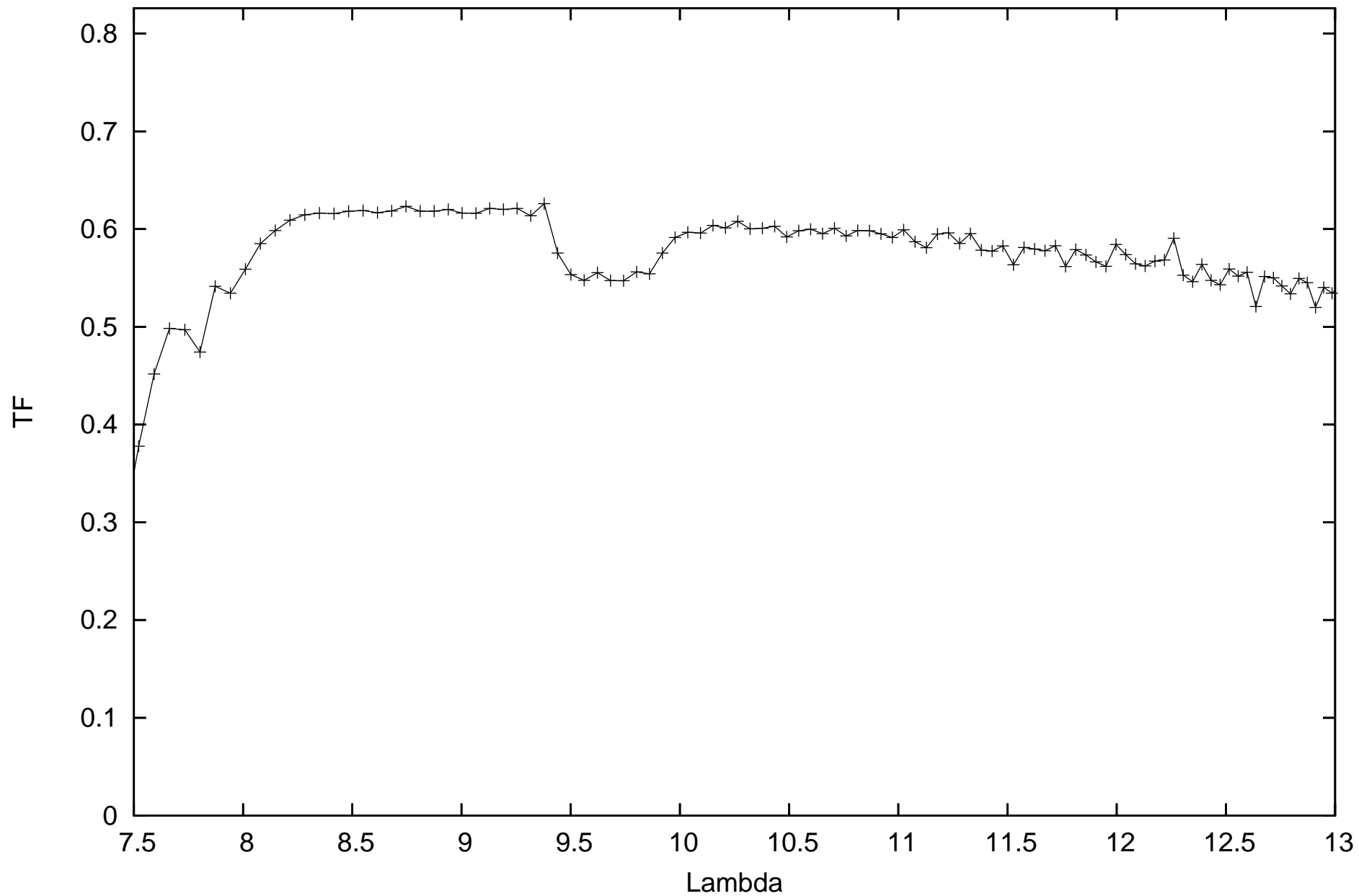
calHIP19038_flux1.83316_diam1.9_r.MIDI.2013-12-20T02_55_12.000_U3U4
