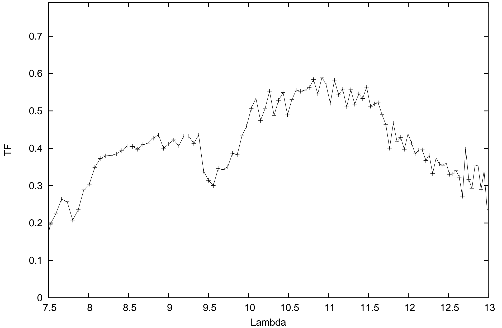
calHIP18597_flux0.324993_diam4.526808_r.MIDI.2013-09-17T06_46_31.000_G111
