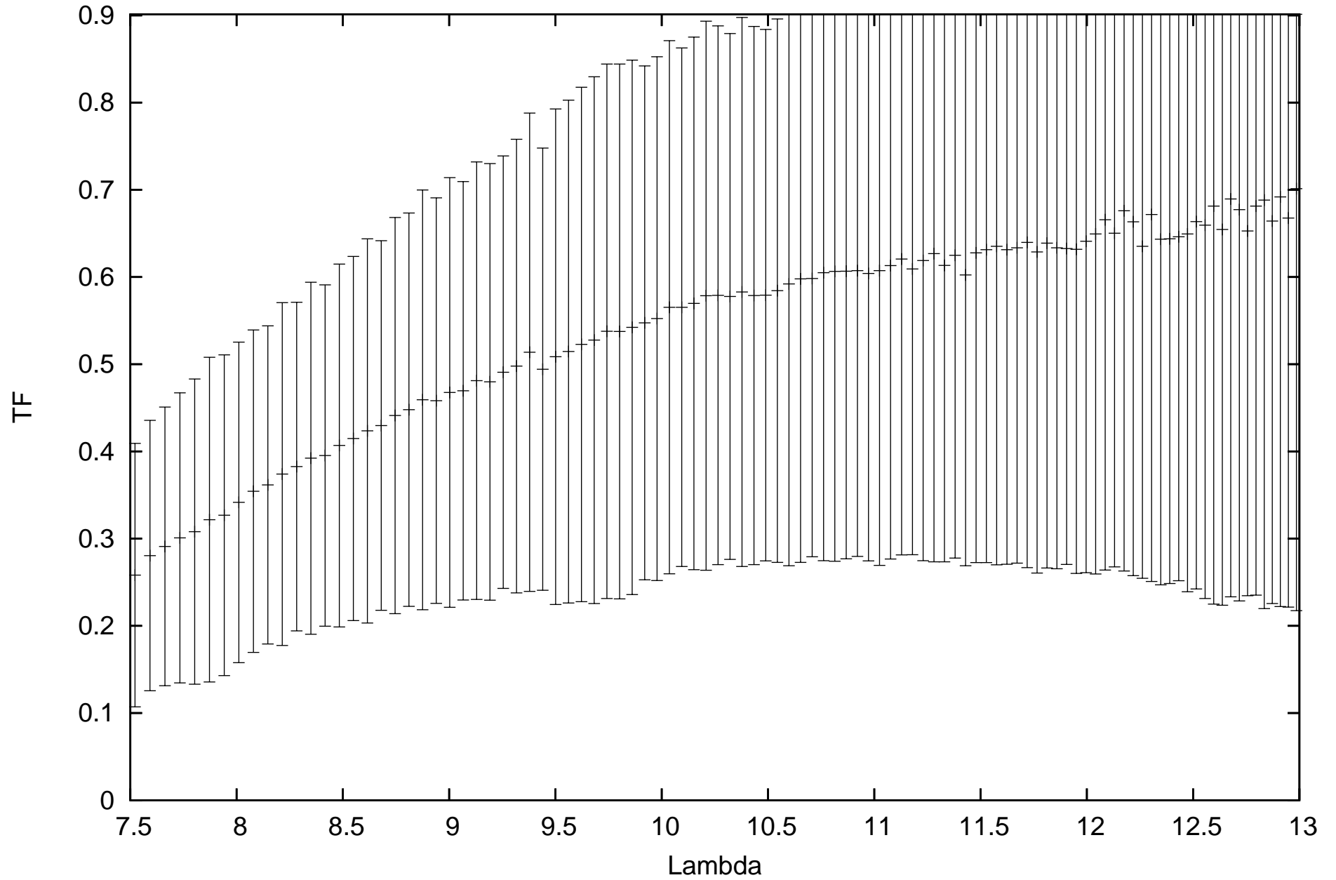
calHIP14135_flux-1.95419_diam12.27_r.MIDI.2013-01-07T01_47_59.000_K0G1
