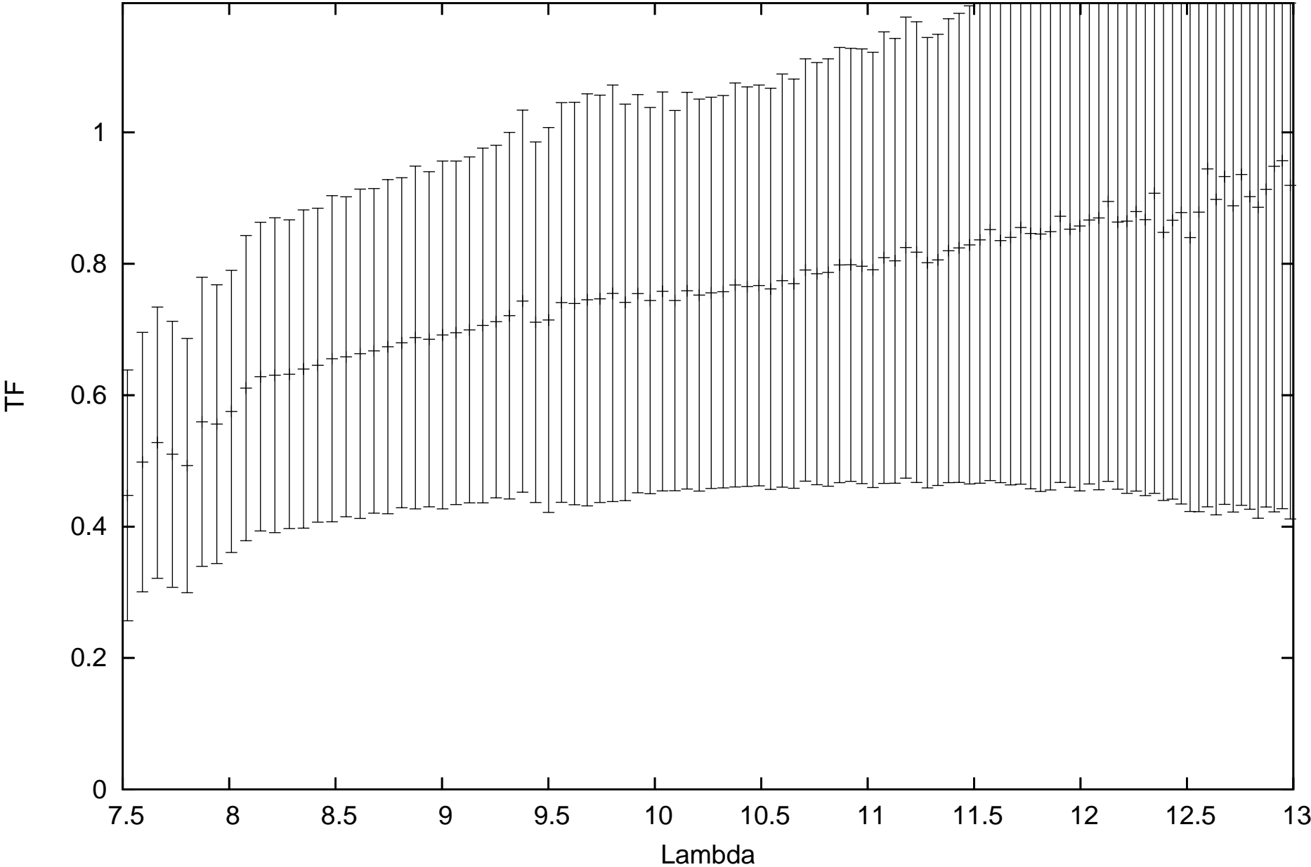
calHIP115830_flux1.69691_diam2.104183_r.MIDI.2013-08-19T07_54_33.000_U3U4
