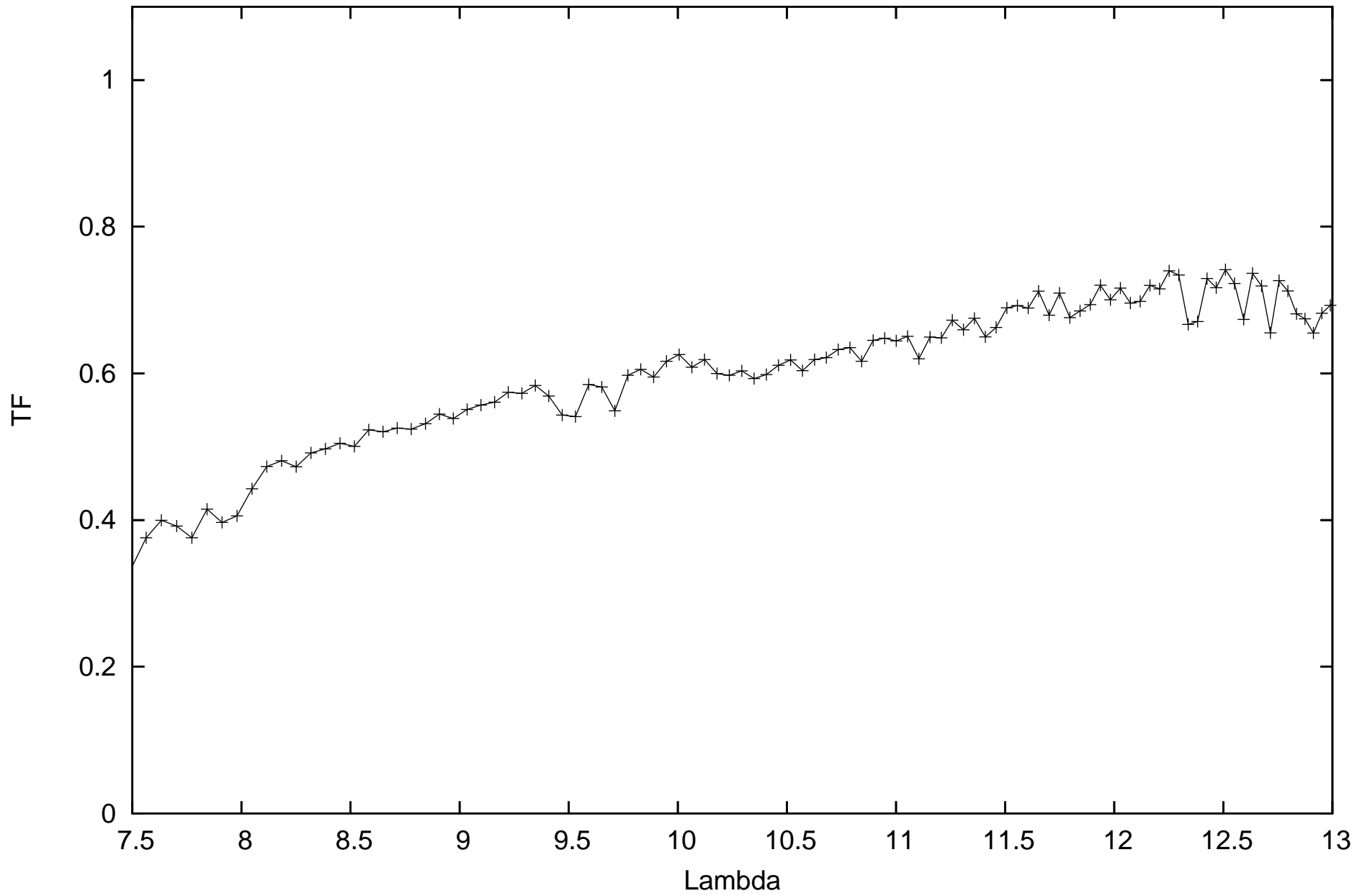
calHIP112748_flux1.25758_diam2.46_r.MIDI.2013-10-24T00_34_46.932_U2U3
