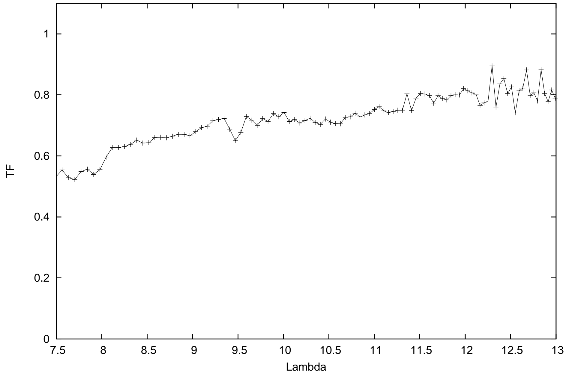
calHIP112440_flux1.47348_diam2.22_r.MIDI.2013-10-24T01_07_08.932_U2U3
