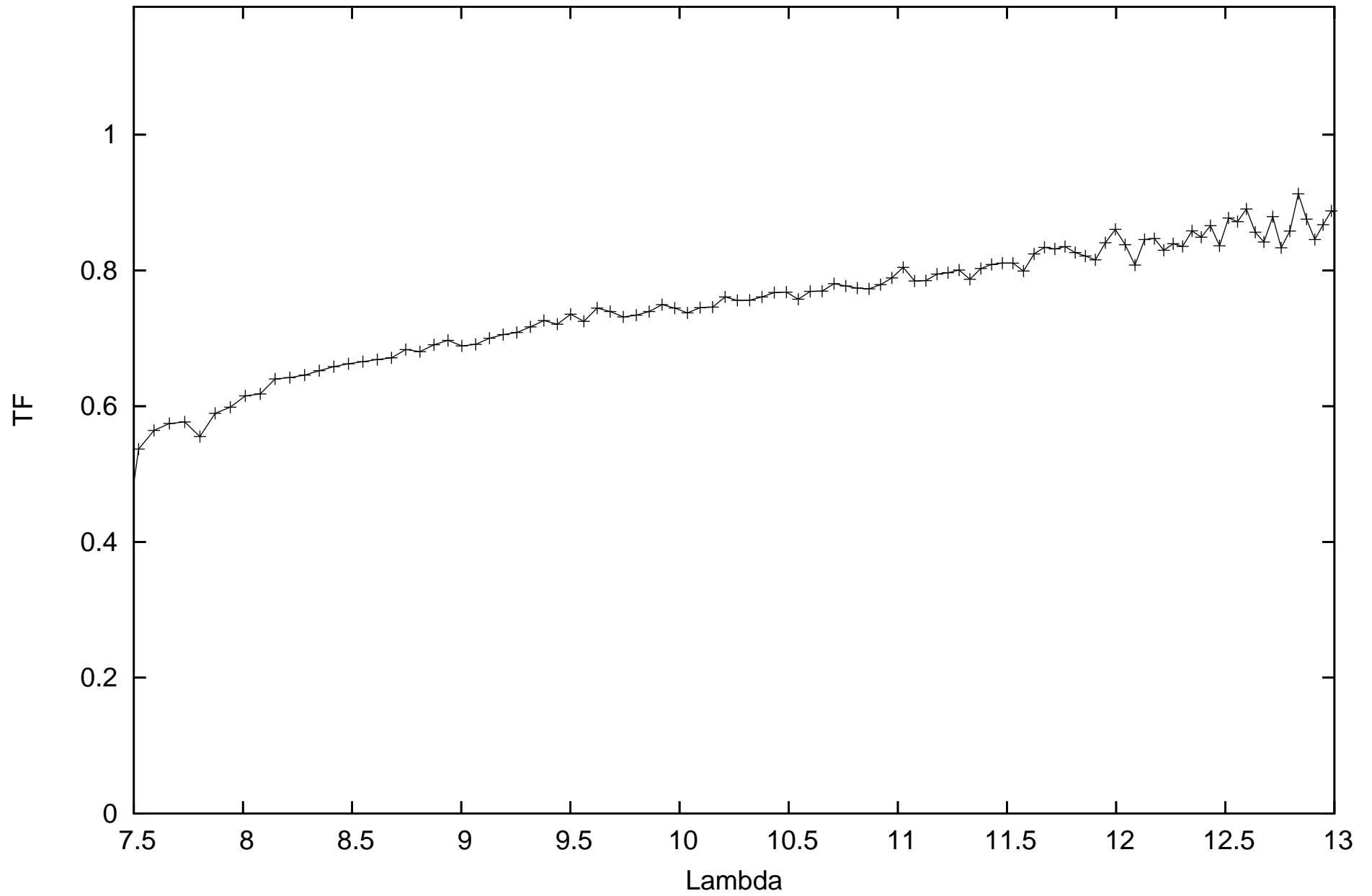
calHIP110997_flux1.58908_diam2.11_r.MIDI.2013-12-15T00_34_13.000_U1U2
