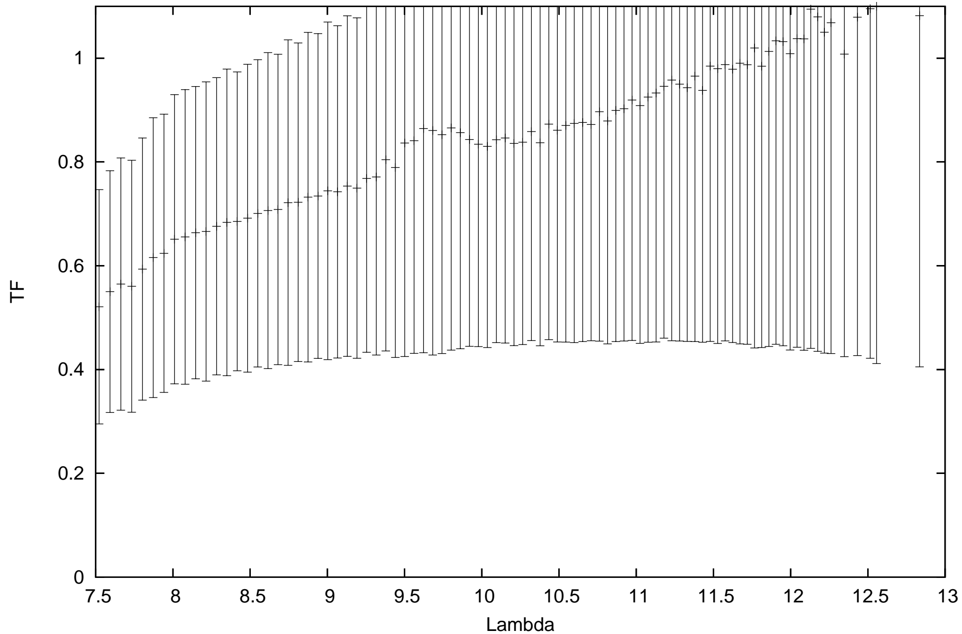
calHIP110997_flux1.58908_diam2.11_r.MIDI.2013-10-20T02_17_17.000_U1U3
