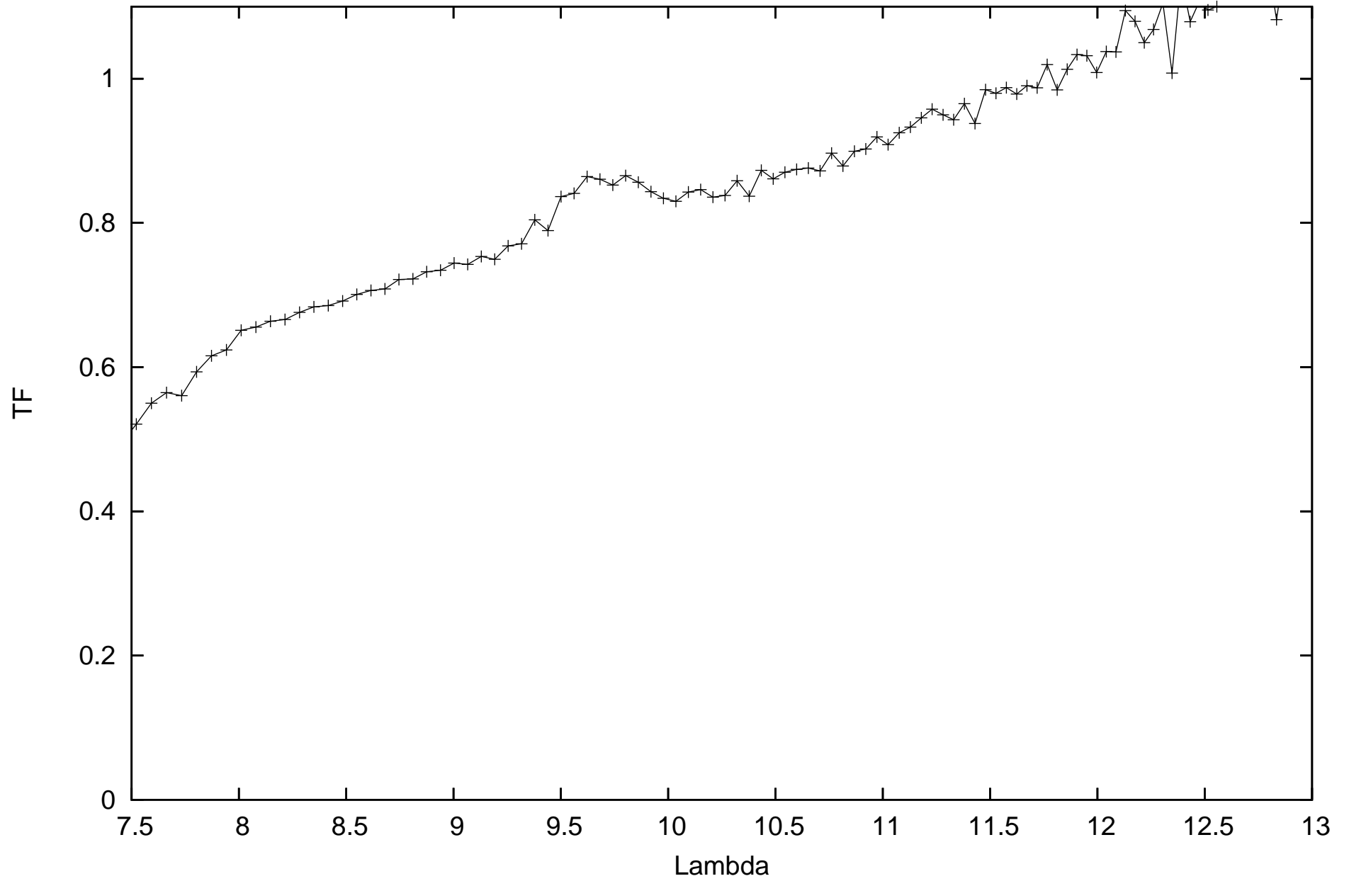
calHIP110997_flux1.58908_diam2.11_r.MIDI.2013-10-20T02_17_17.000_U1U3
