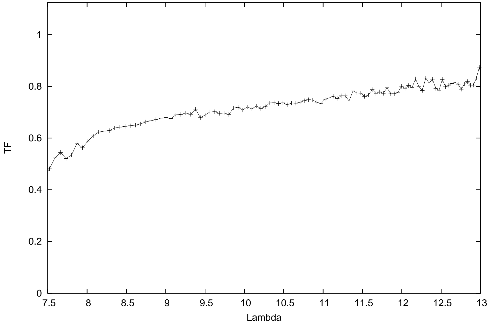
calHIP110997_flux1.58908_diam2.11_r.MIDI.2013-08-19T06_34_31.000_U3U4
