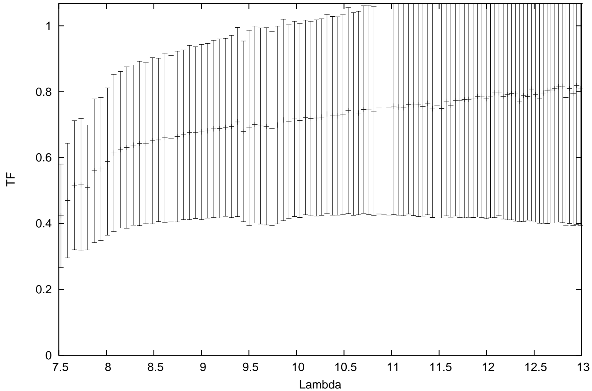
calHIP110997_flux1.58908_diam2.11_r.MIDI.2013-08-18T07_14_09.000_U3U4
