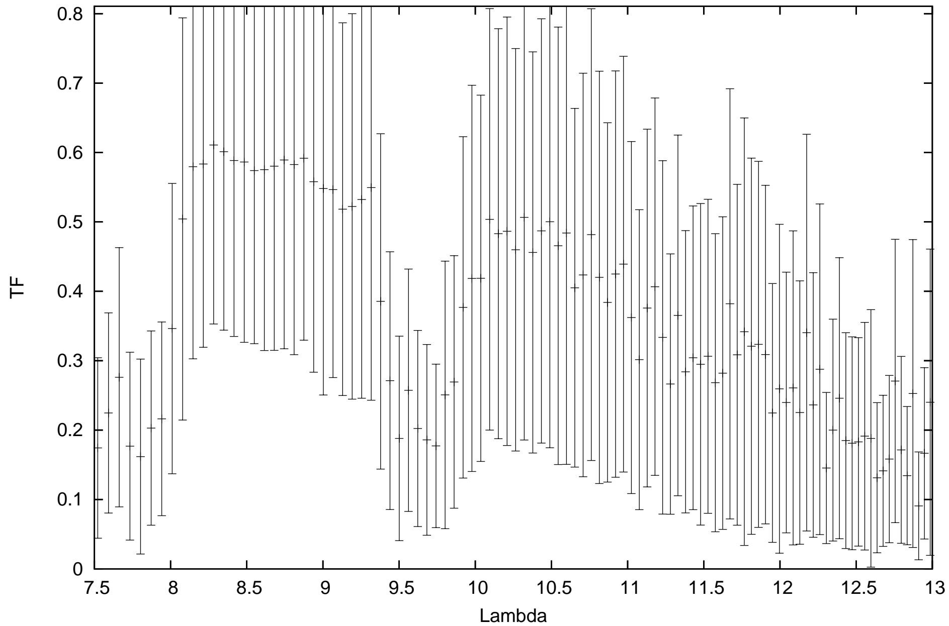
calHD98292_flux0.92_diam3.35_r.MIDI.2013-12-30T05_51_56.000_K0J3
