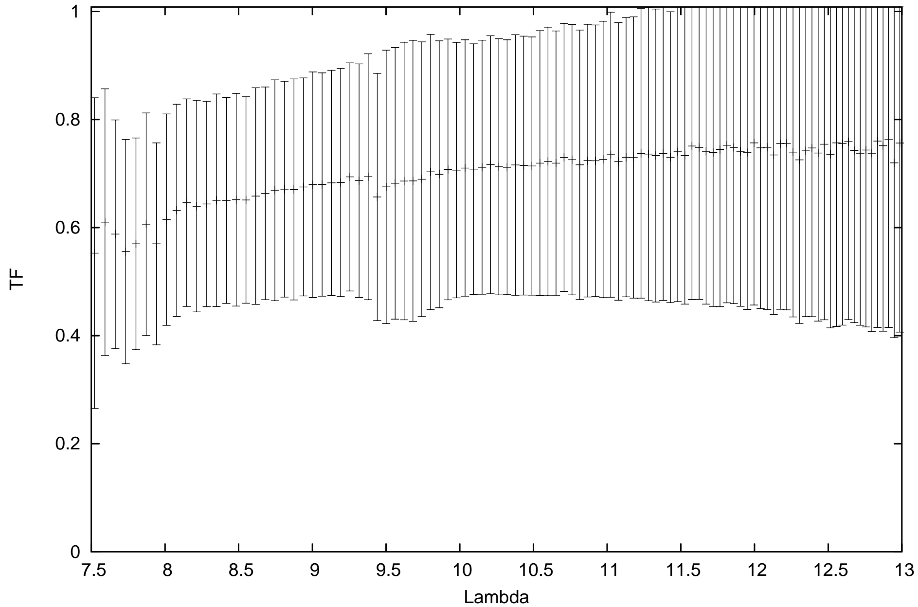
calHD98292_flux0.92_diam3.35_r.MIDI.2013-03-01T07_05_13.000_U3U4
