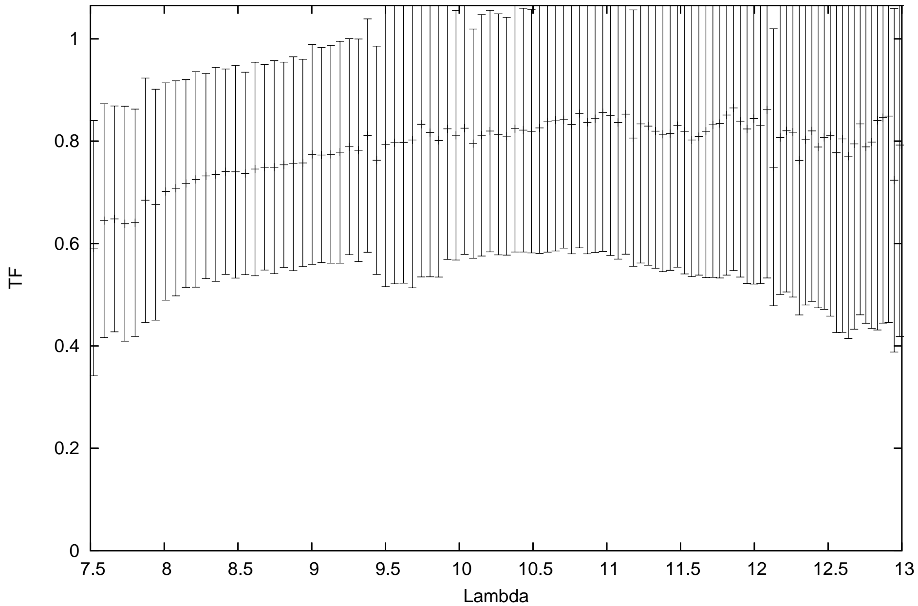
calHD81797_flux-1.49_diam9.14_r.MIDI.2013-11-28T05_50_14.000_D0C1
