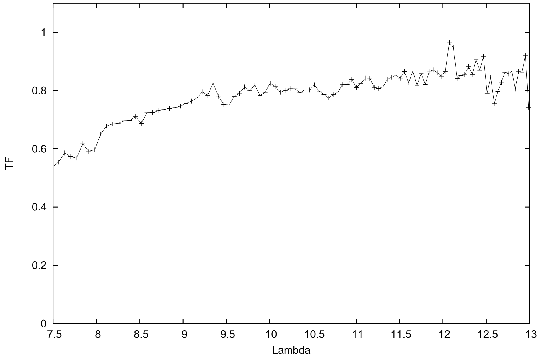
calHD81797_flux-1.49_diam9.14_r.MIDI.2013-04-13T03_15_28.112_C1A1
