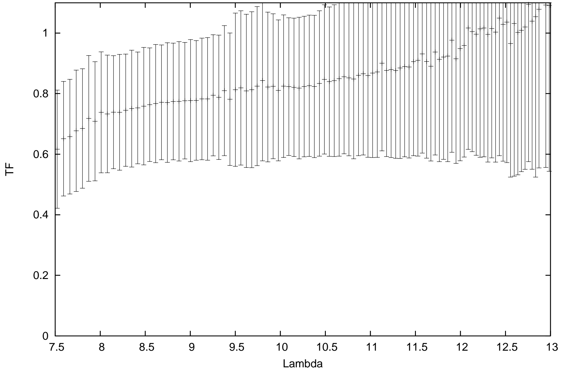
calHD81797_flux-1.49_diam9.14_r.MIDI.2013-03-29T02_21_05.000_D0B2
