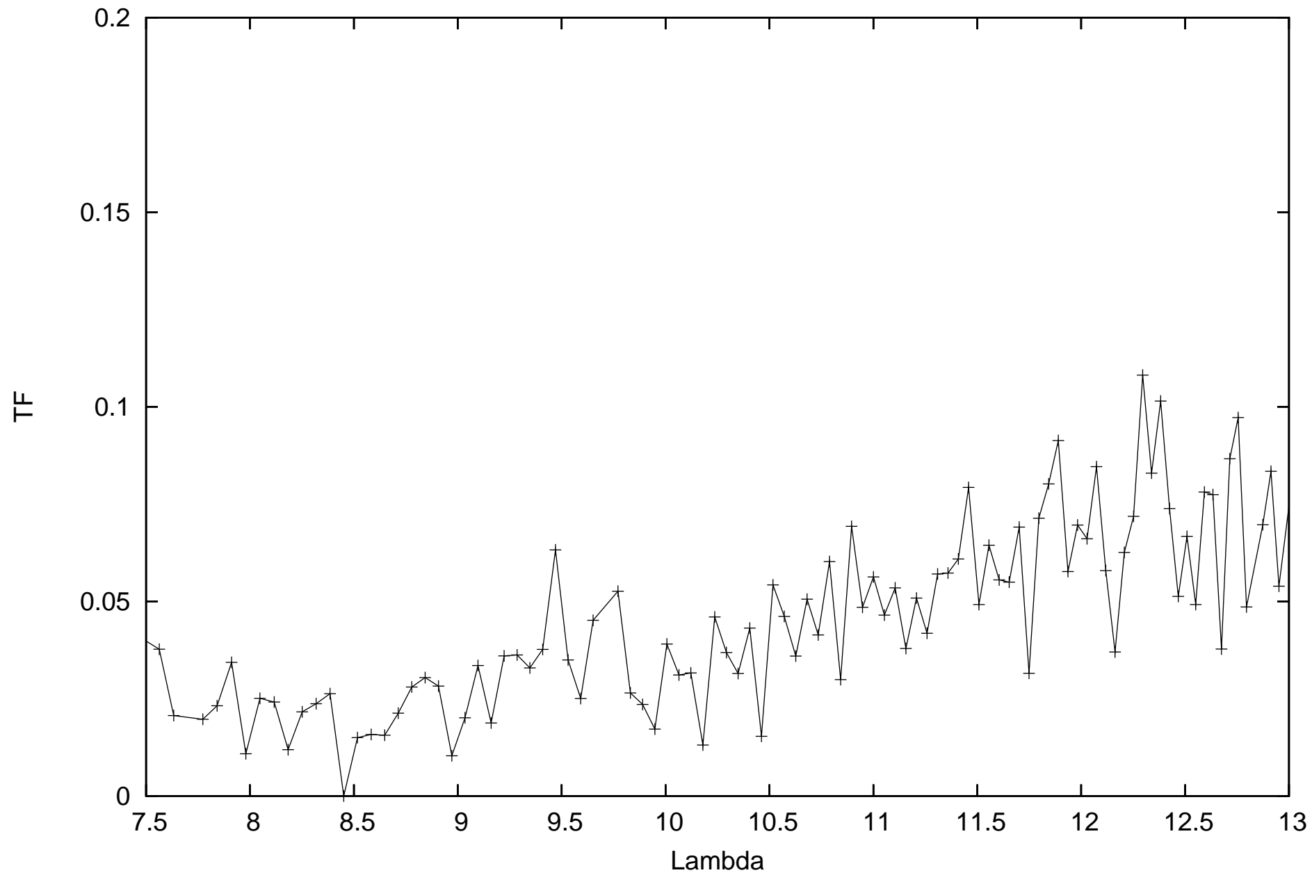
calHD81797_flux-1.49_diam9.14_r.MIDI.2013-02-15T03_08_41.113_H011
