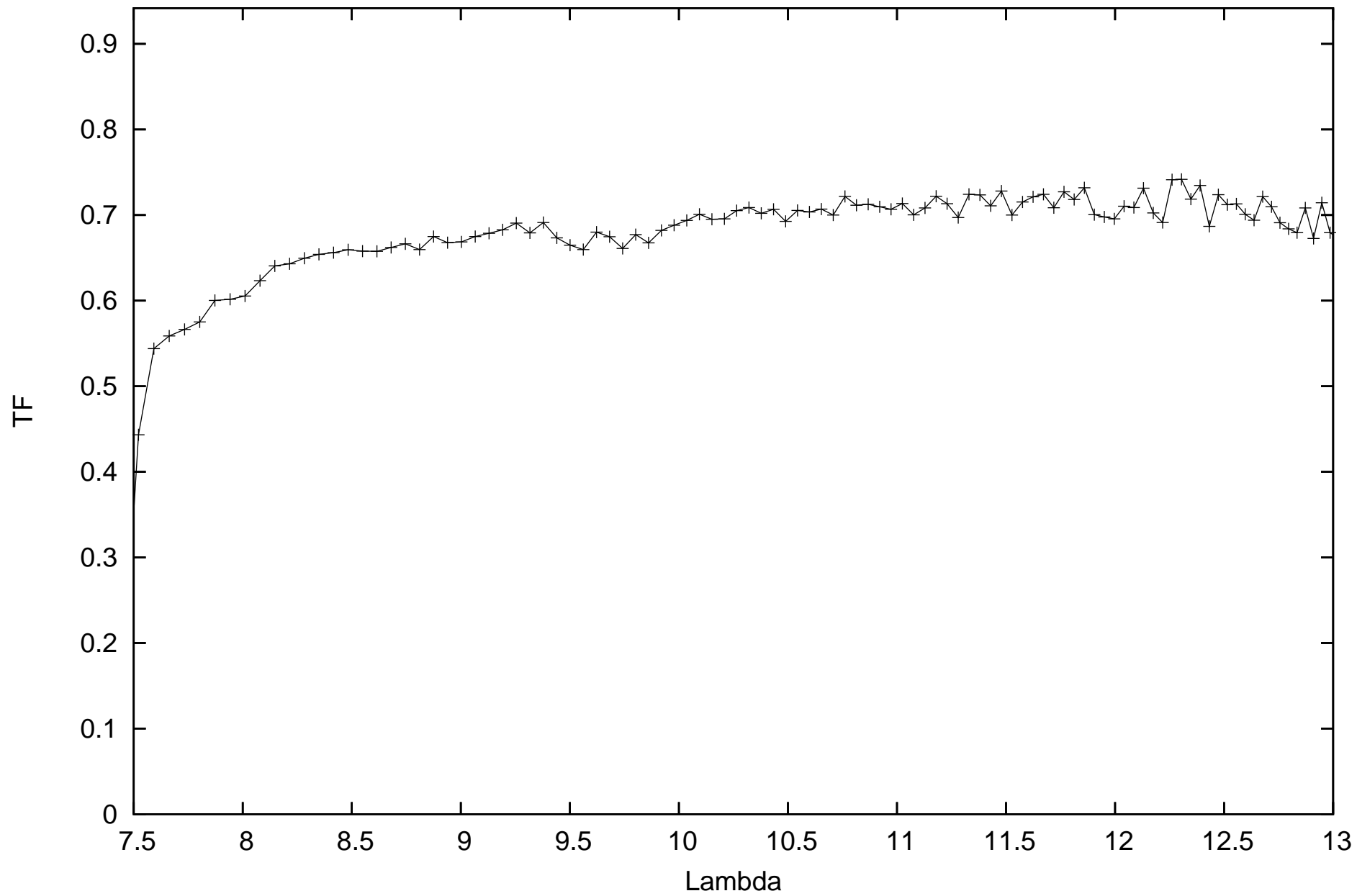
calHD81797_flux-1.49_diam9.14_r.MIDI.2013-02-14T03_56_10.000_H0G1
