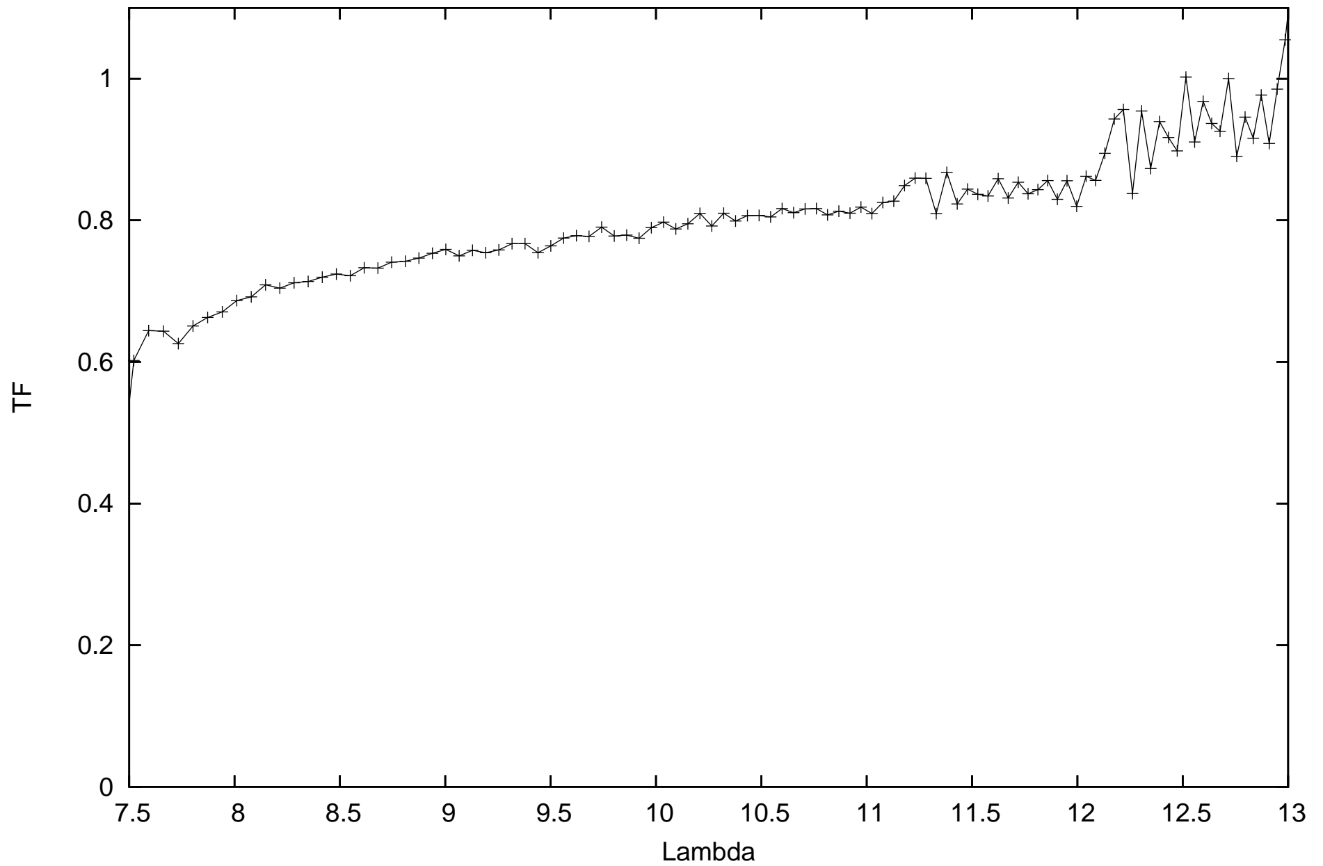
calHD48915_flux-1.39_diam6.09_r.MIDI.2013-03-06T02_30_43.000_G2I1
